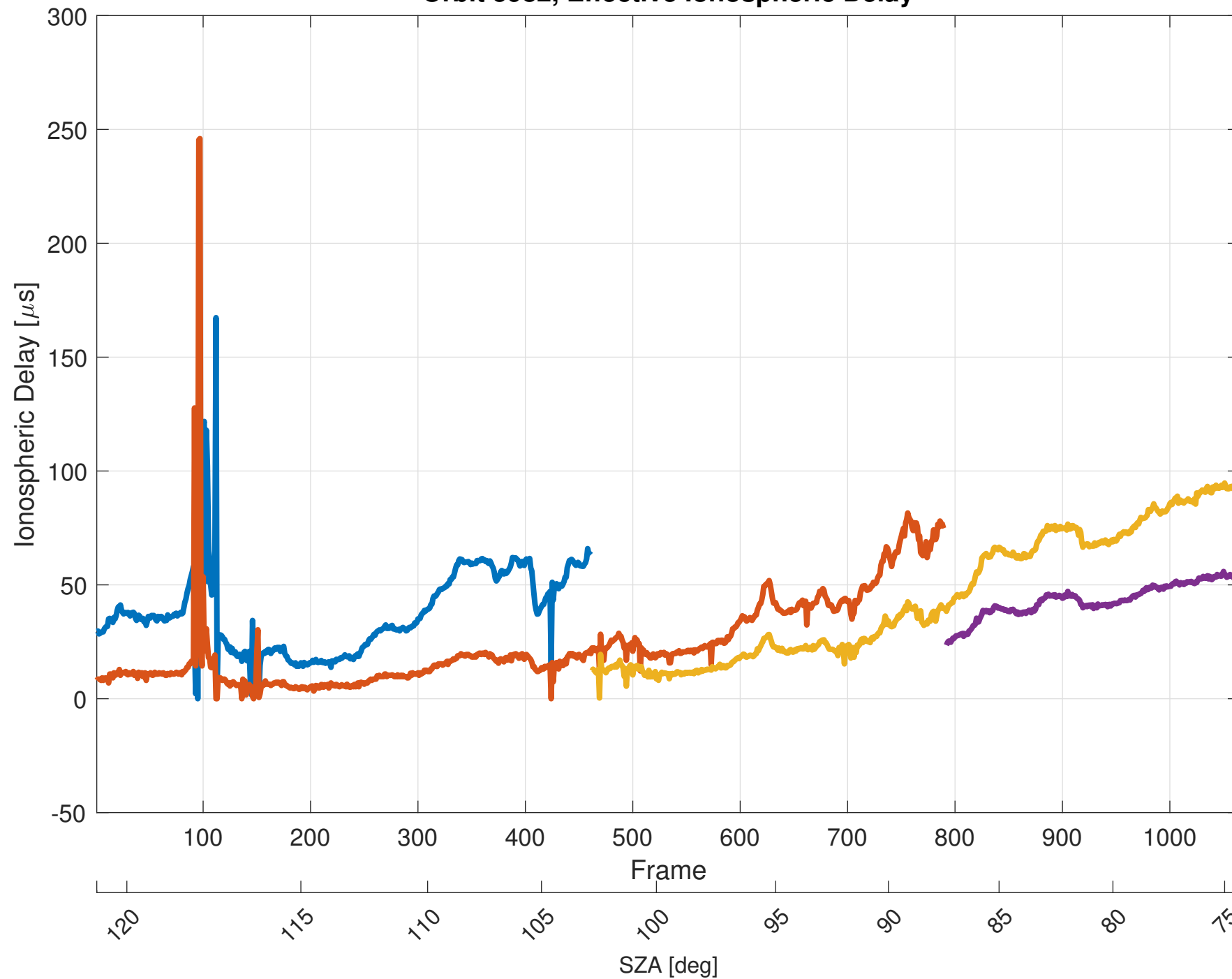
Orbit 5982, Effective Ionospheric Delay
