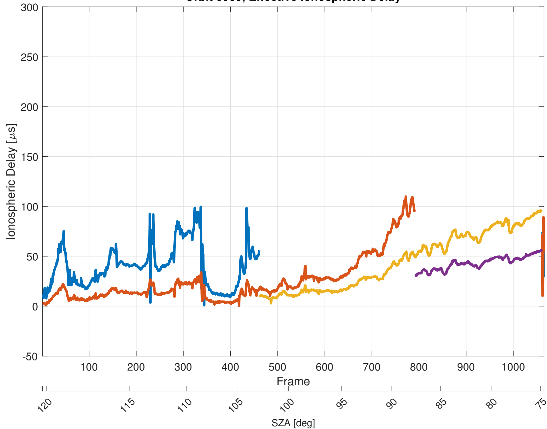
Orbit 5985, Effective Ionospheric Delay
