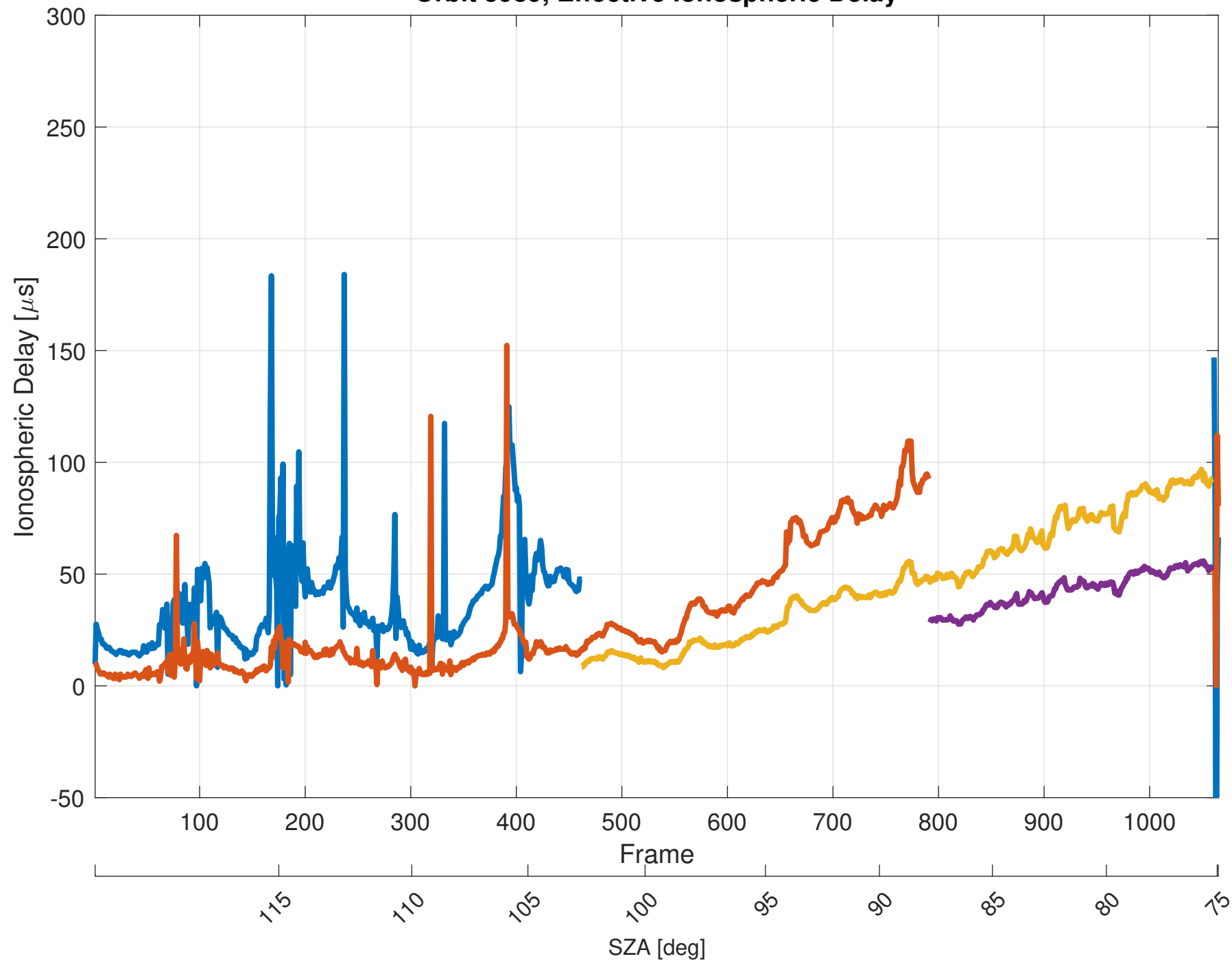
Orbit 5989, Effective Ionospheric Delay
