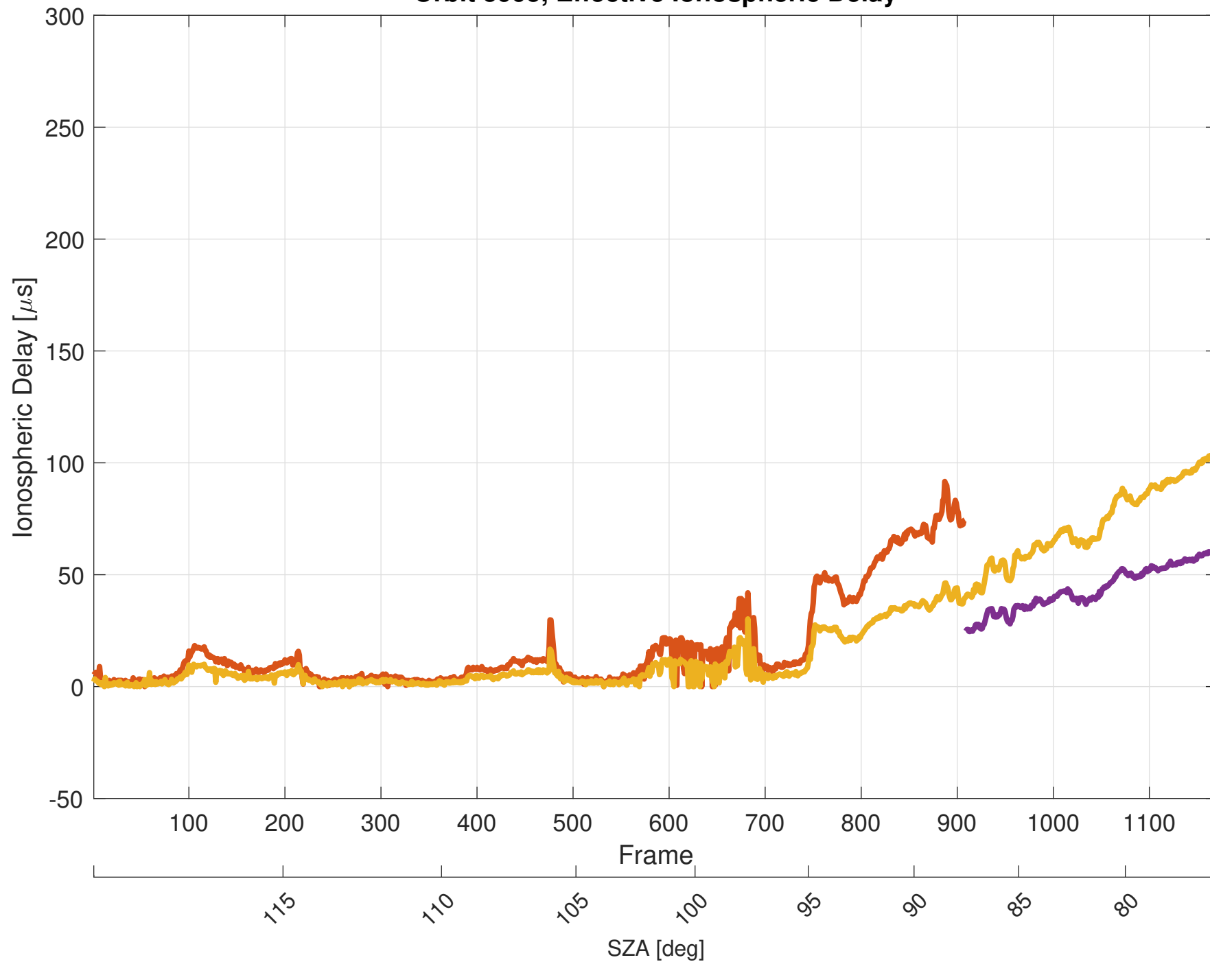
Orbit 5995, Effective Ionospheric Delay
