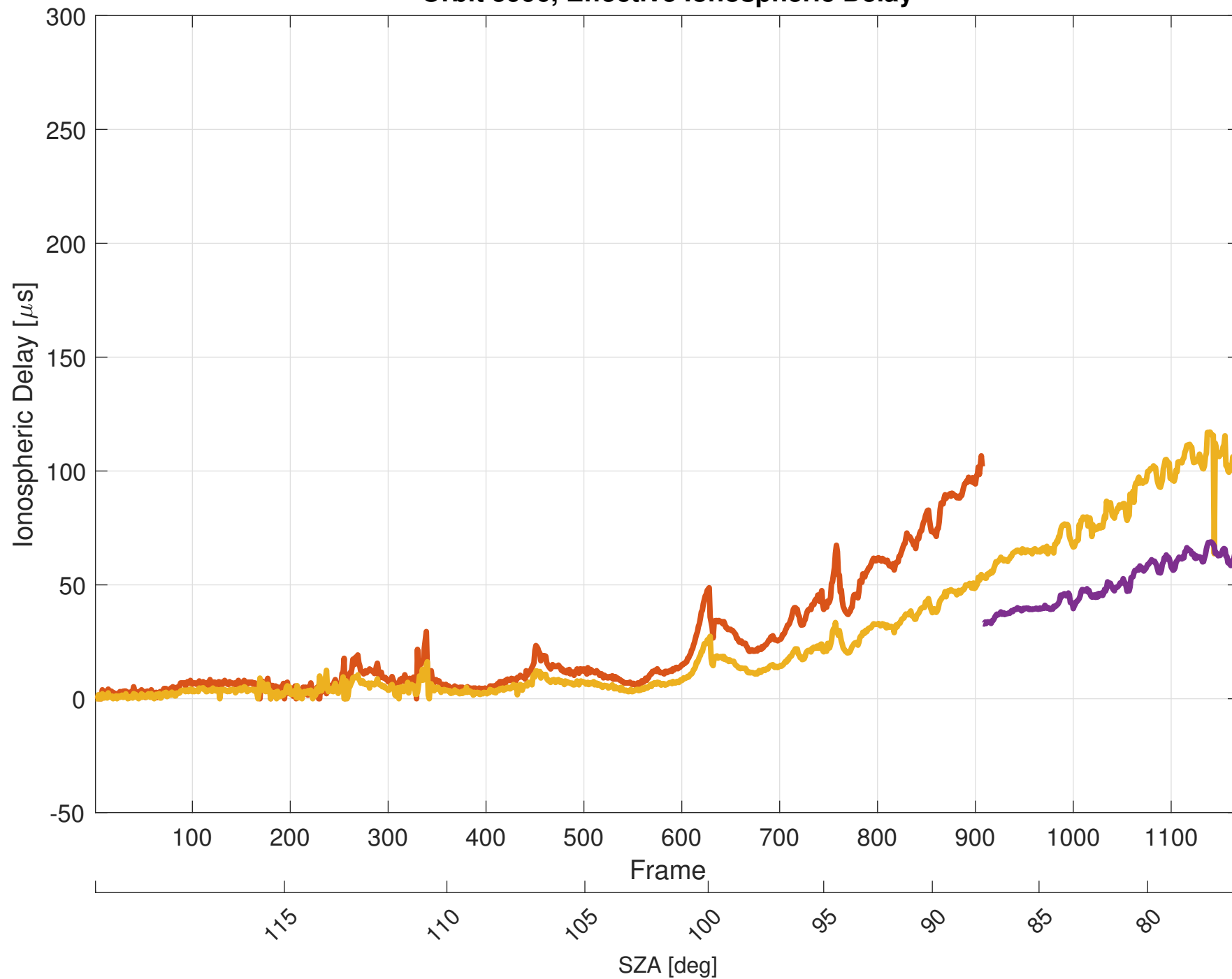
Orbit 5996, Effective Ionospheric Delay
