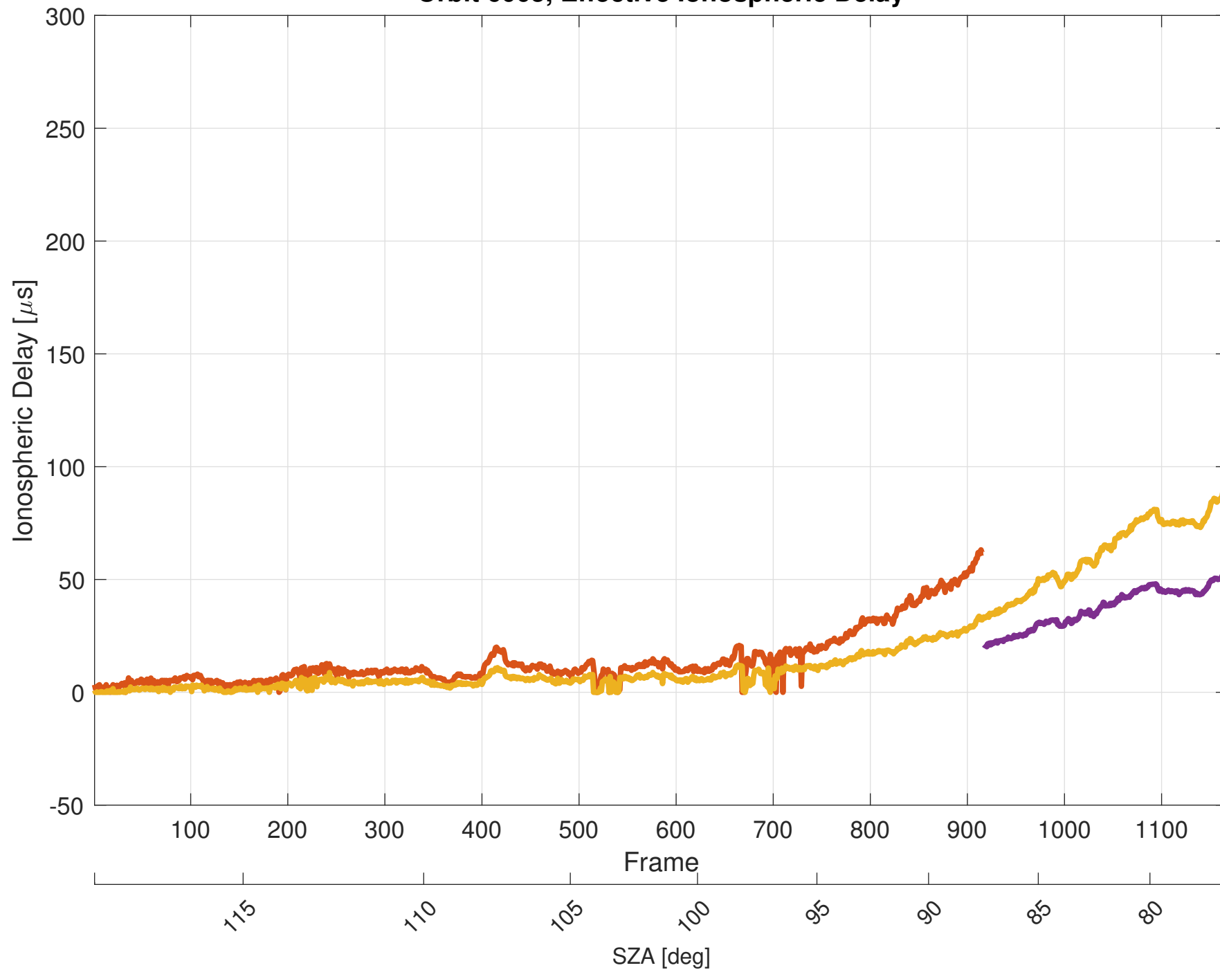
Orbit 6005, Effective Ionospheric Delay
