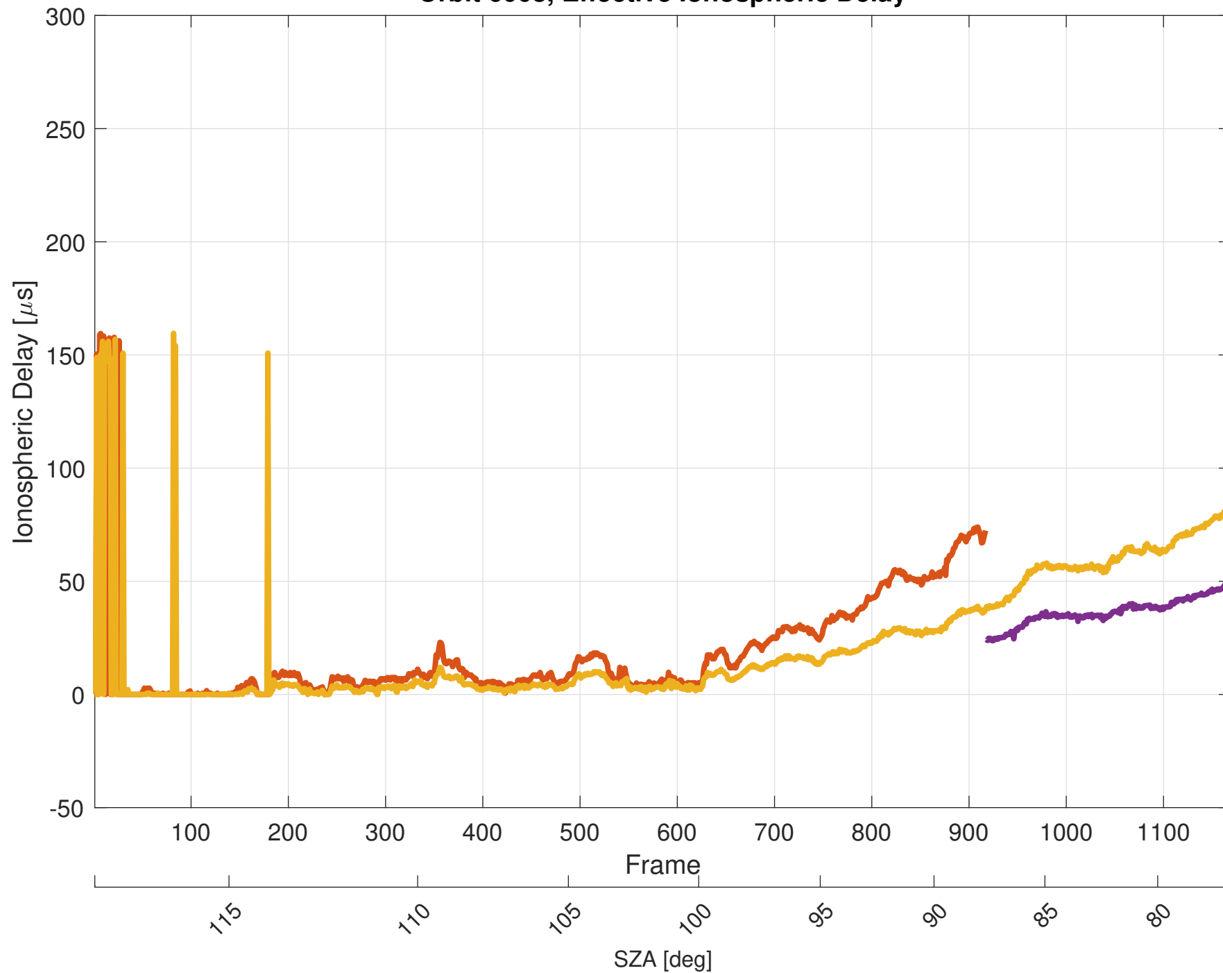
Orbit 6008, Effective Ionospheric Delay
