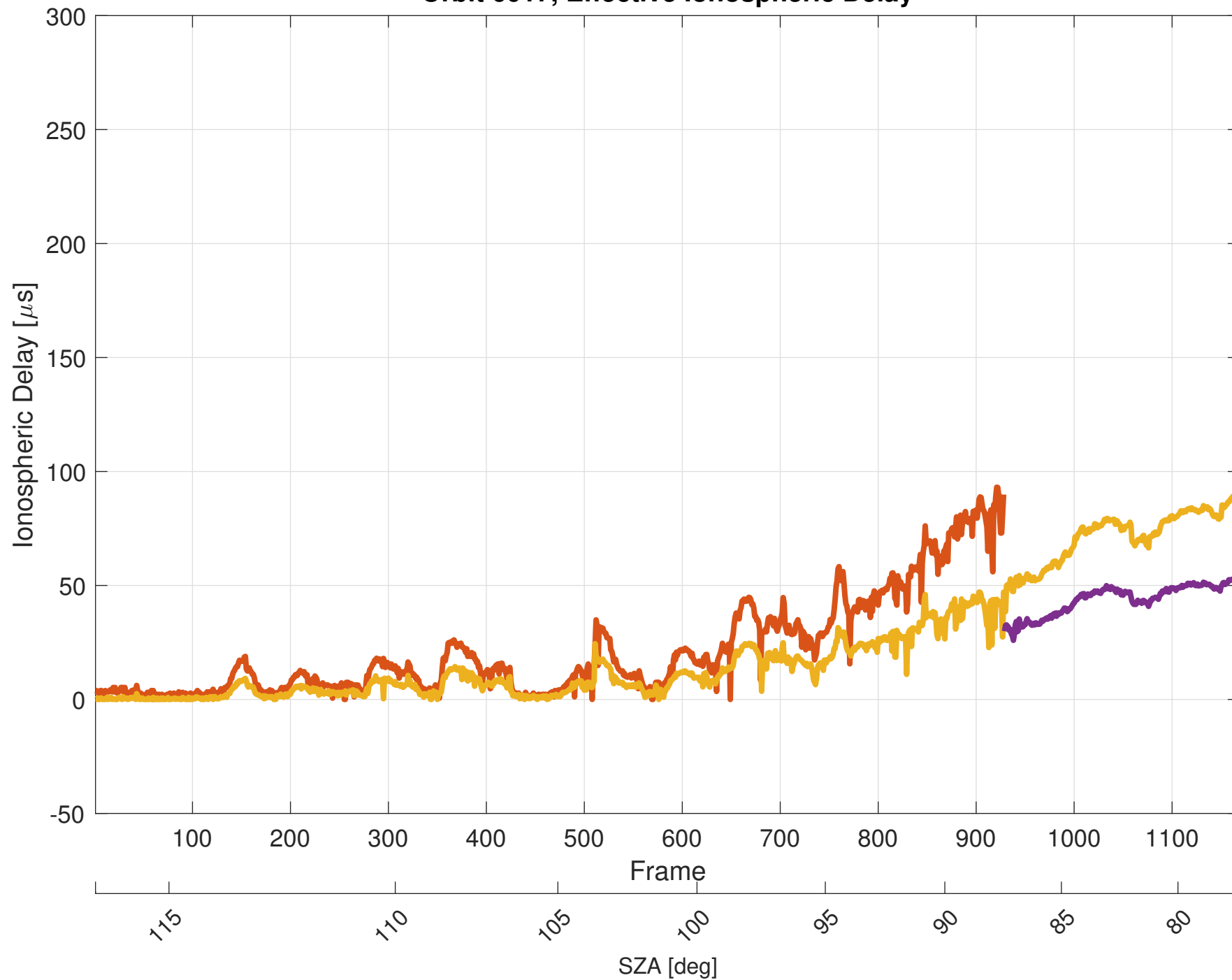
Orbit 6017, Effective Ionospheric Delay
