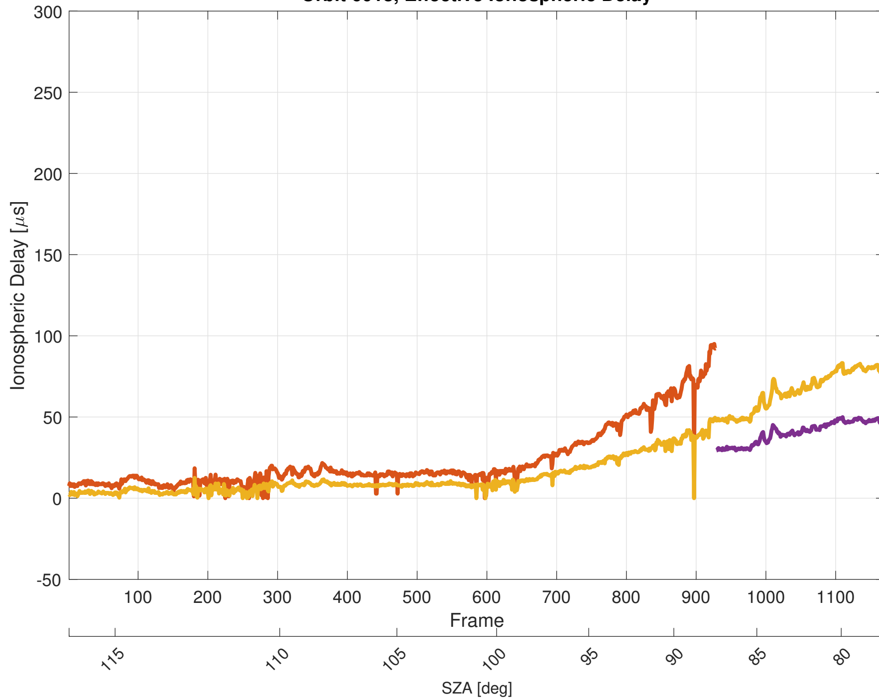
Orbit 6018, Effective Ionospheric Delay
