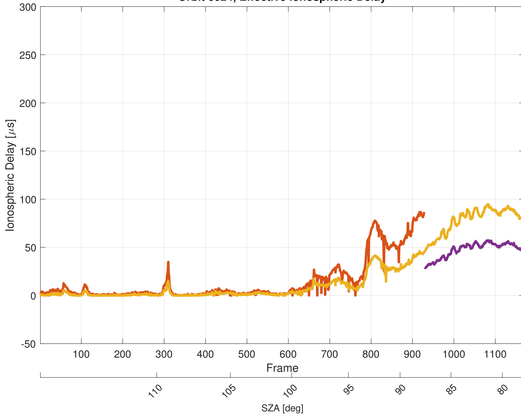
Orbit 6024, Effective Ionospheric Delay
