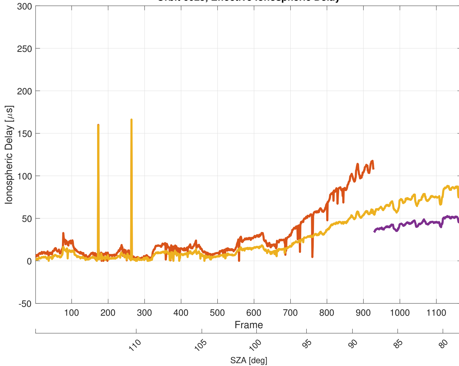
Orbit 6025, Effective Ionospheric Delay
