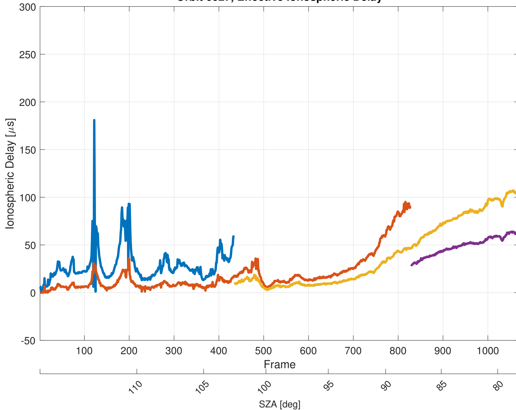
Orbit 6027, Effective Ionospheric Delay
