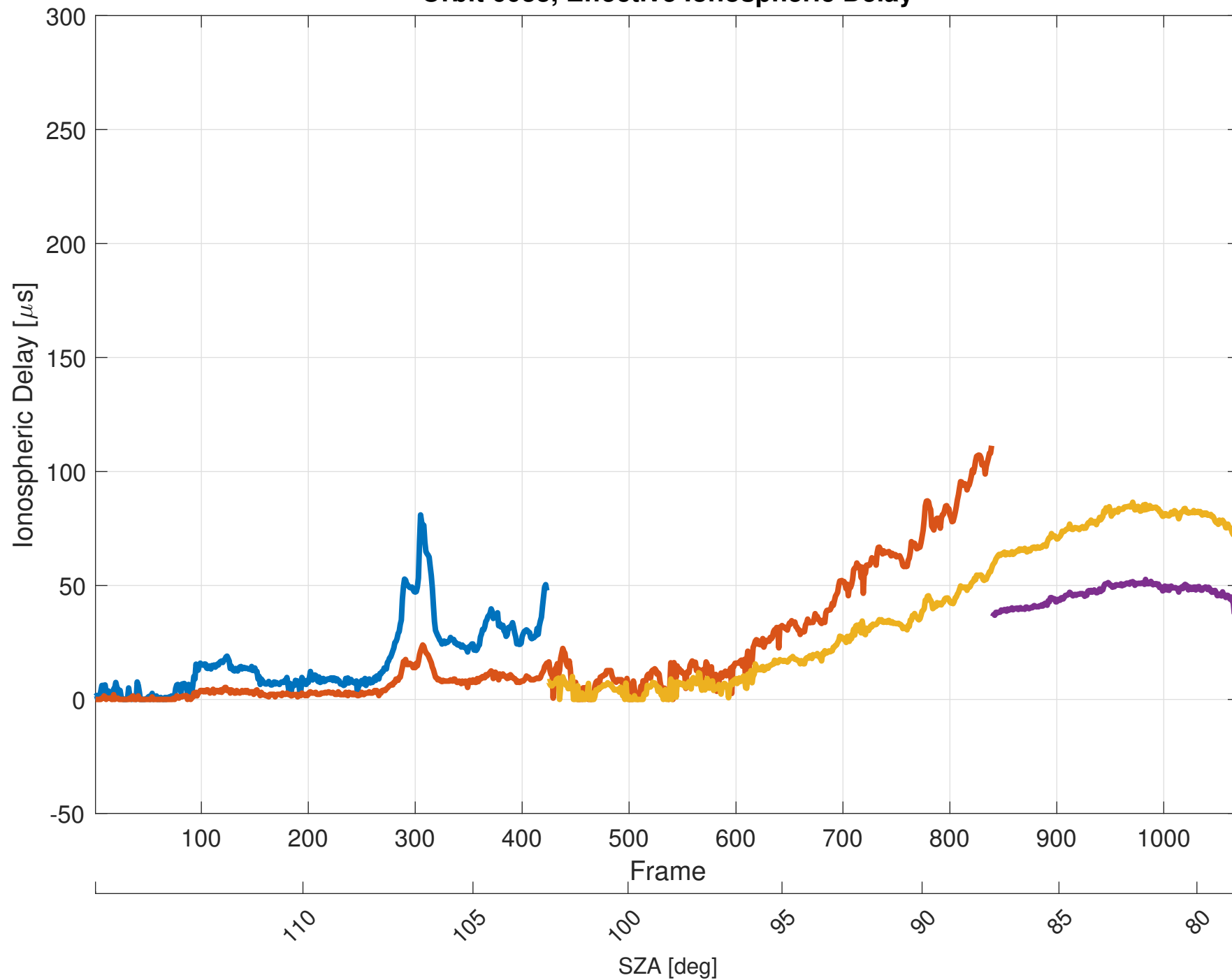
Orbit 6033, Effective Ionospheric Delay
