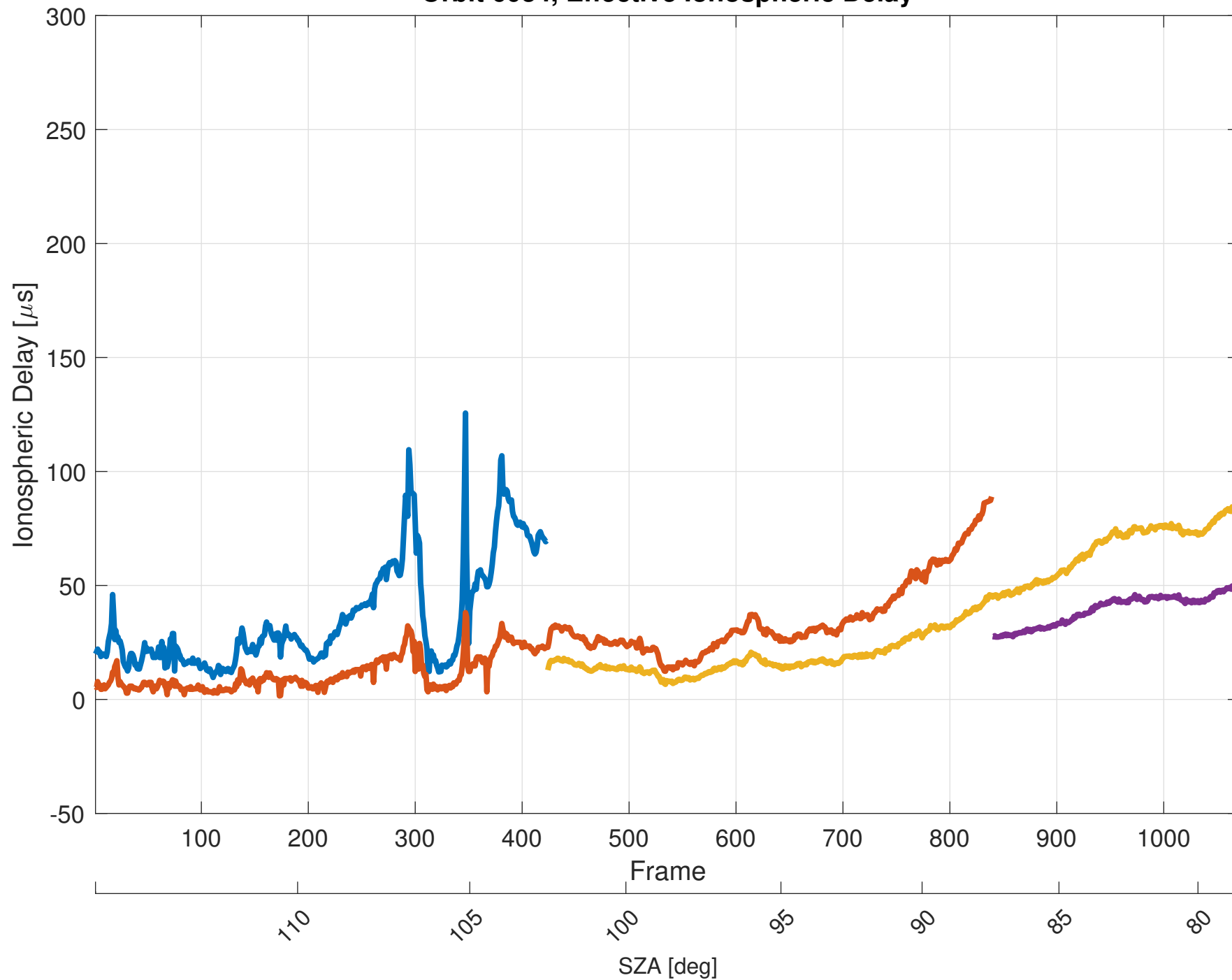
Orbit 6034, Effective Ionospheric Delay
