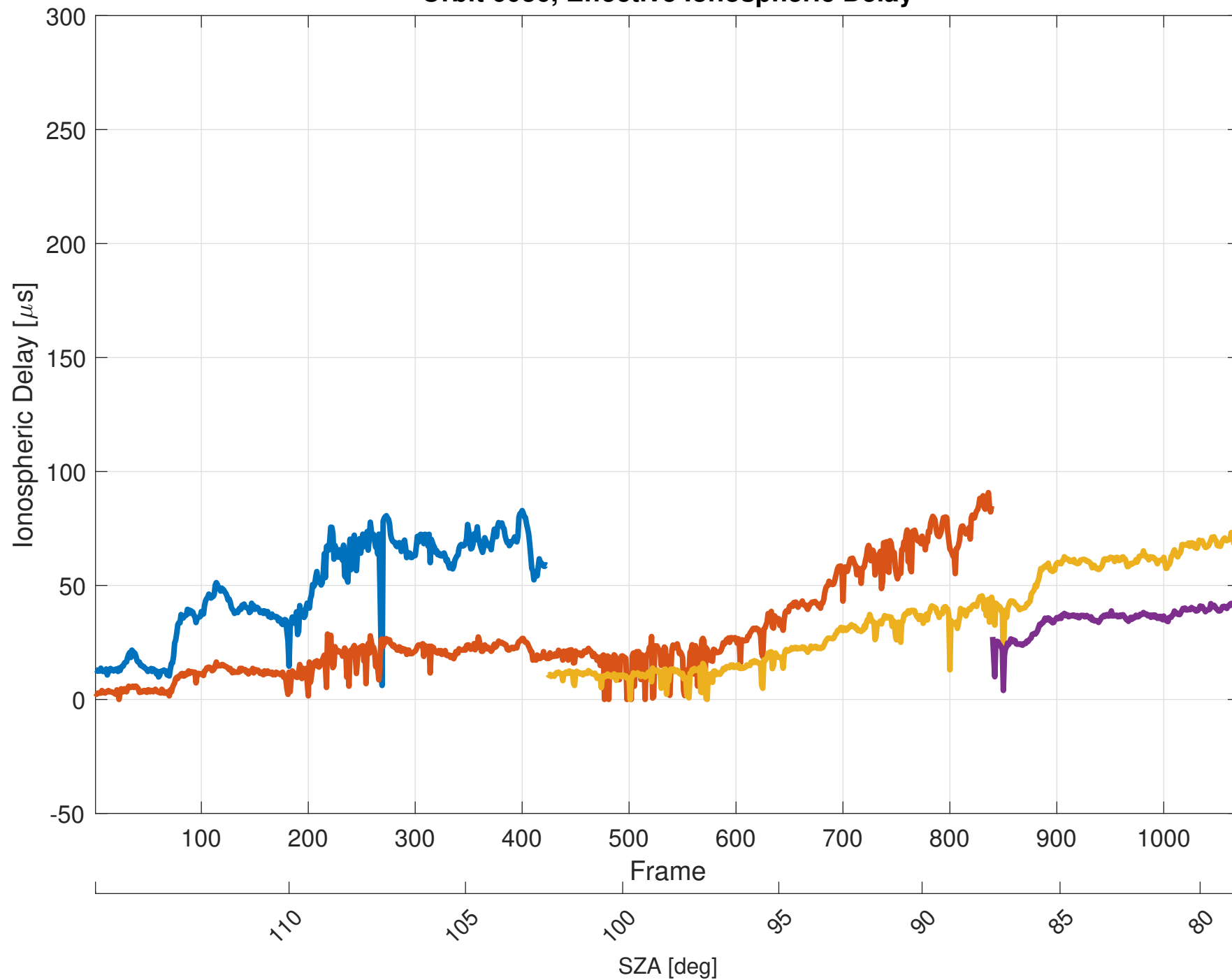
Orbit 6036, Effective Ionospheric Delay
