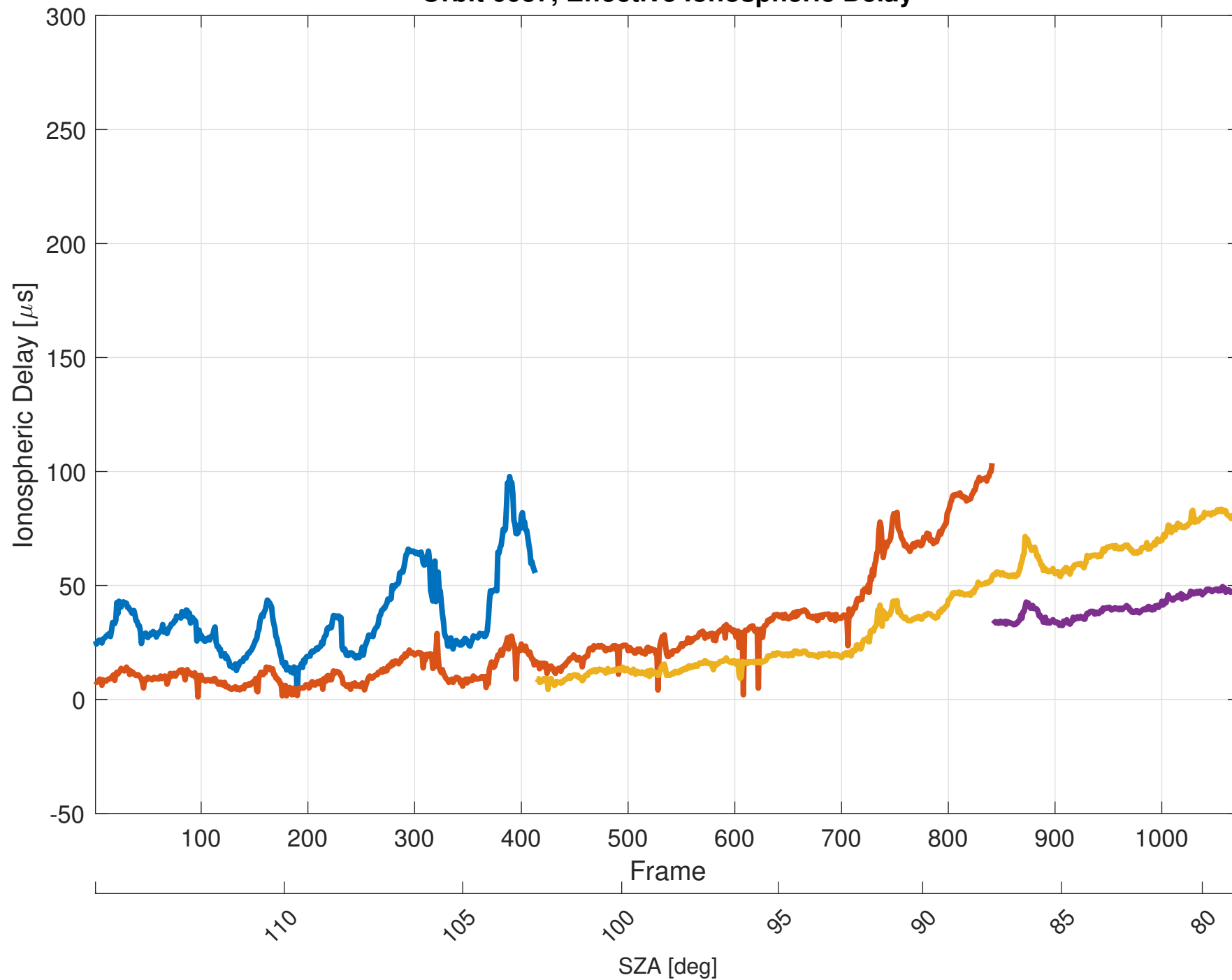
Orbit 6037, Effective Ionospheric Delay
