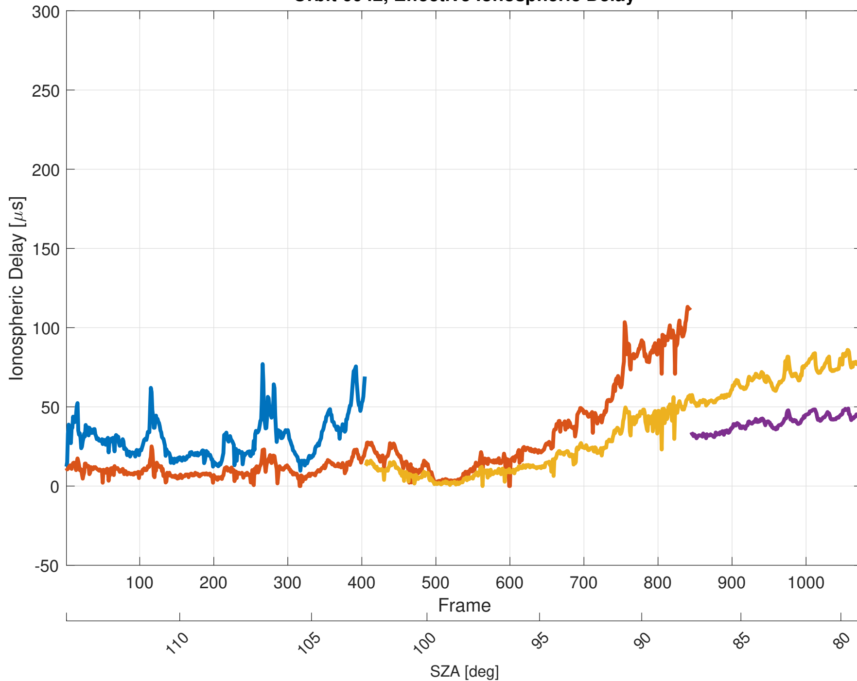
Orbit 6042, Effective Ionospheric Delay
