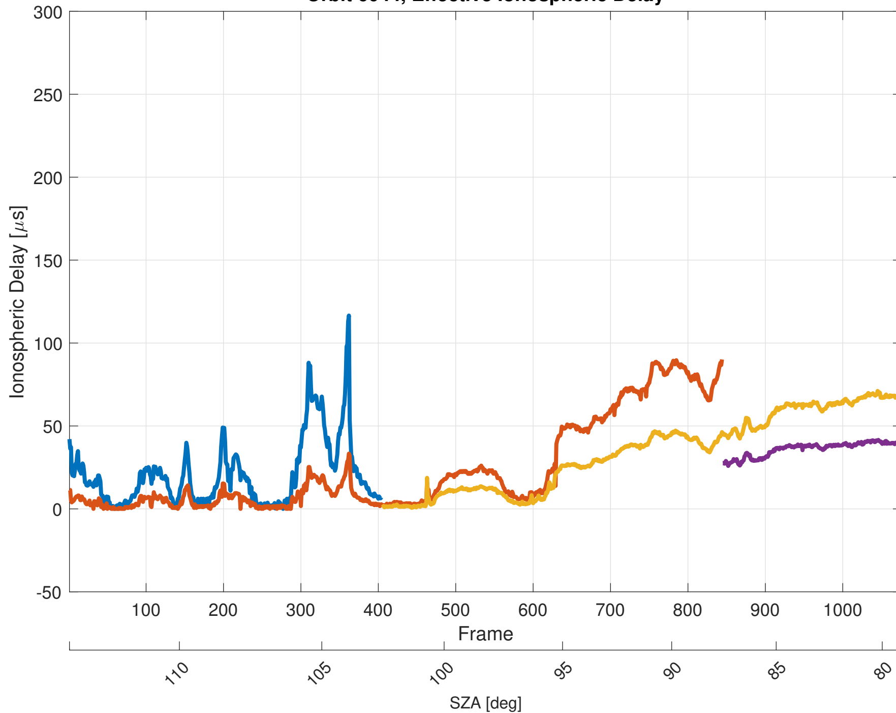
Orbit 6044, Effective Ionospheric Delay
