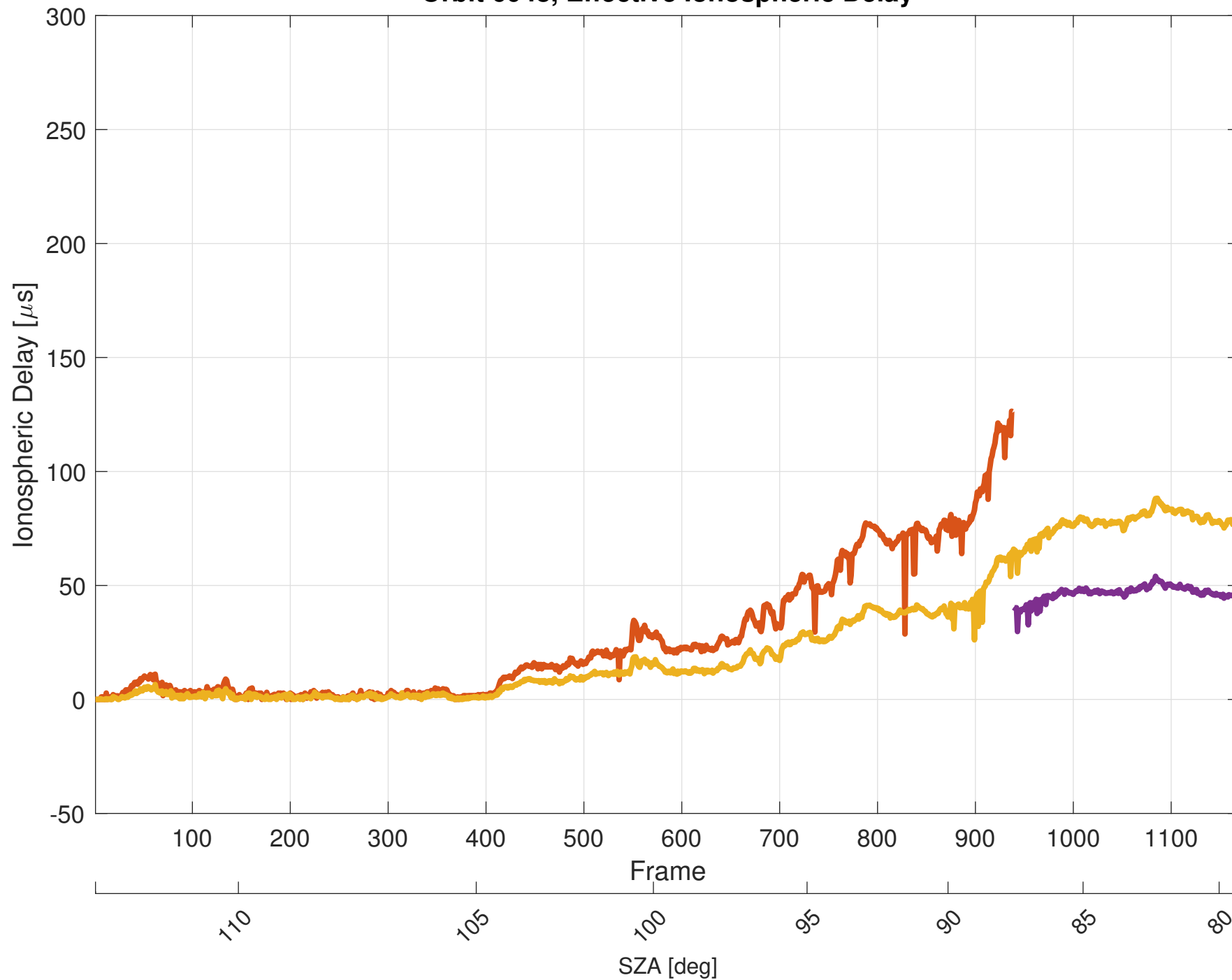
Orbit 6048, Effective Ionospheric Delay
