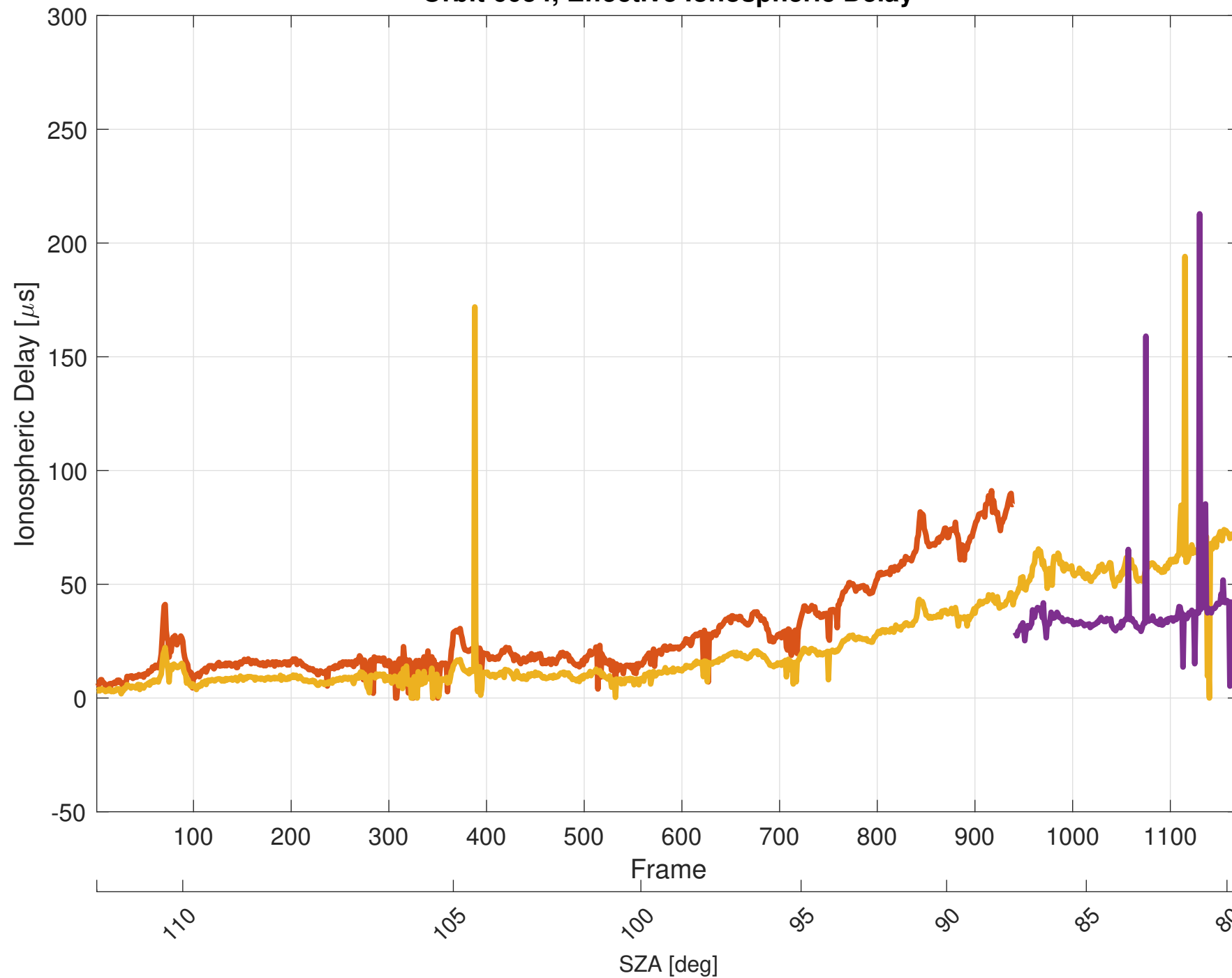
Orbit 6054, Effective Ionospheric Delay
