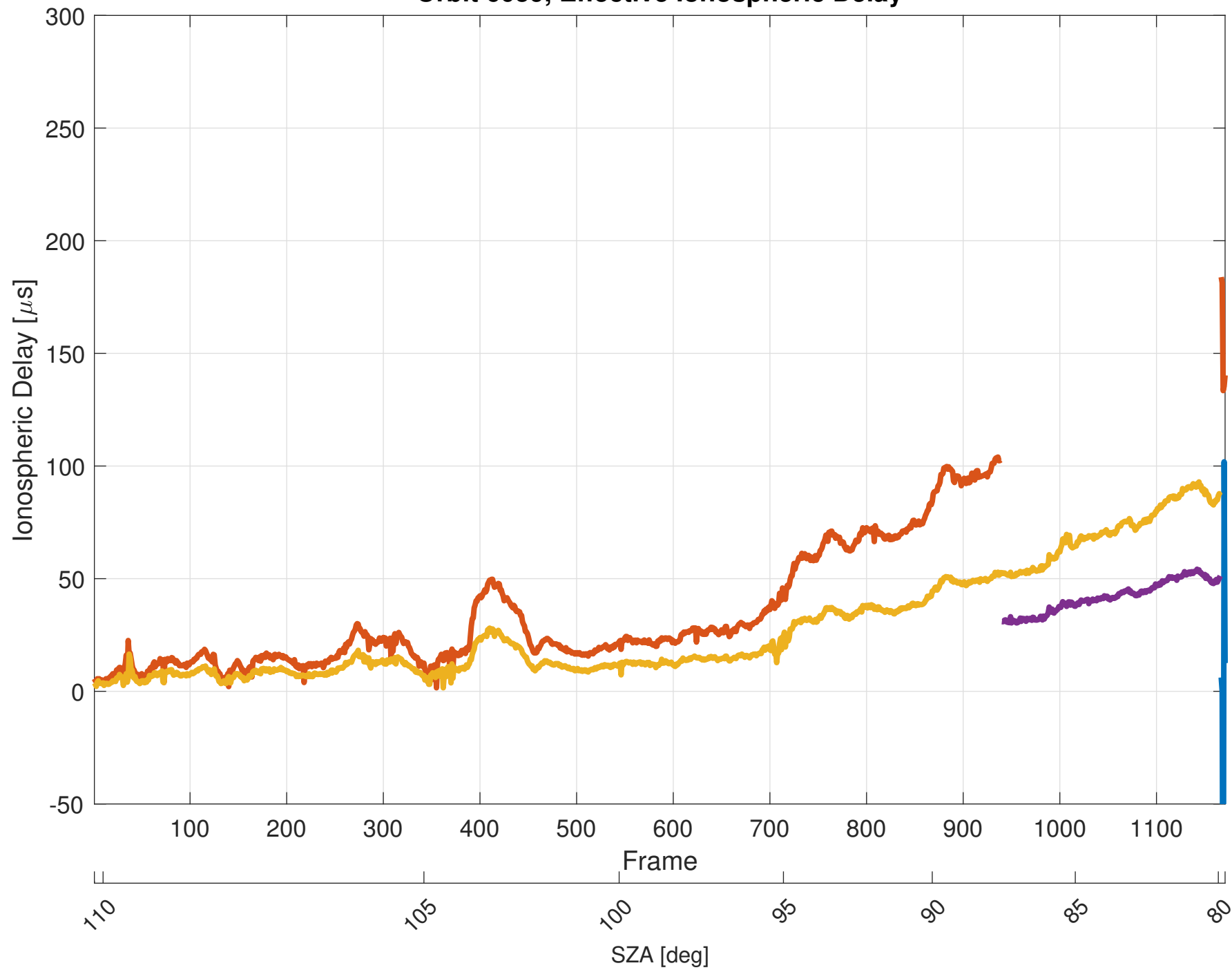
Orbit 6059, Effective Ionospheric Delay
