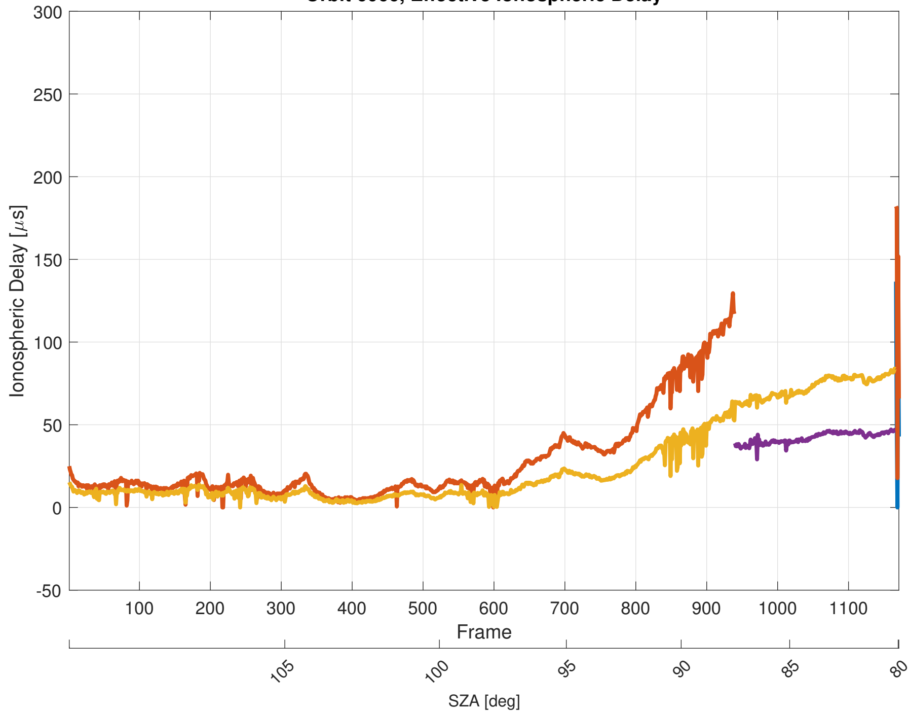
Orbit 6066, Effective Ionospheric Delay
