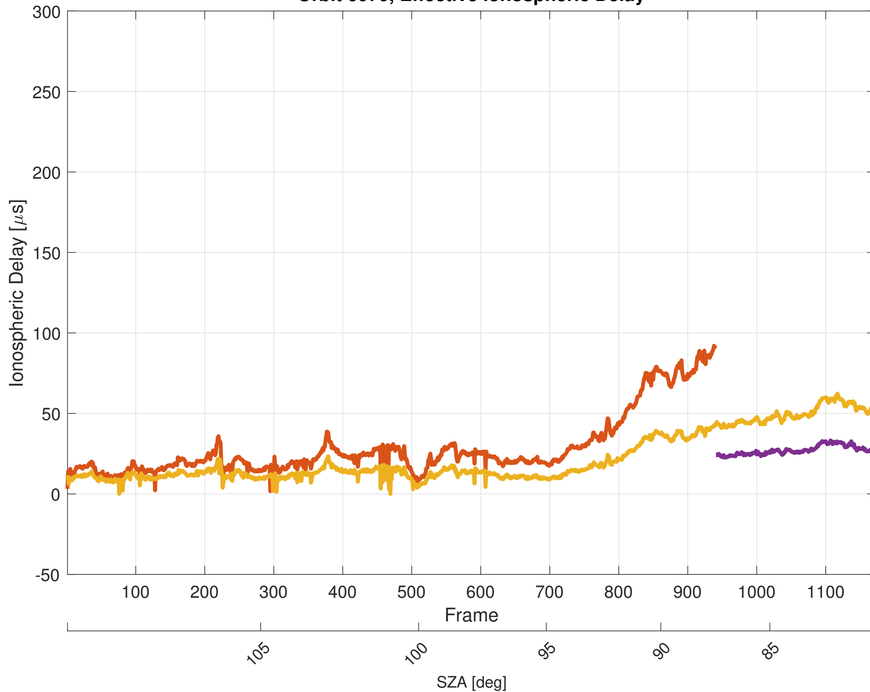
Orbit 6070, Effective Ionospheric Delay
