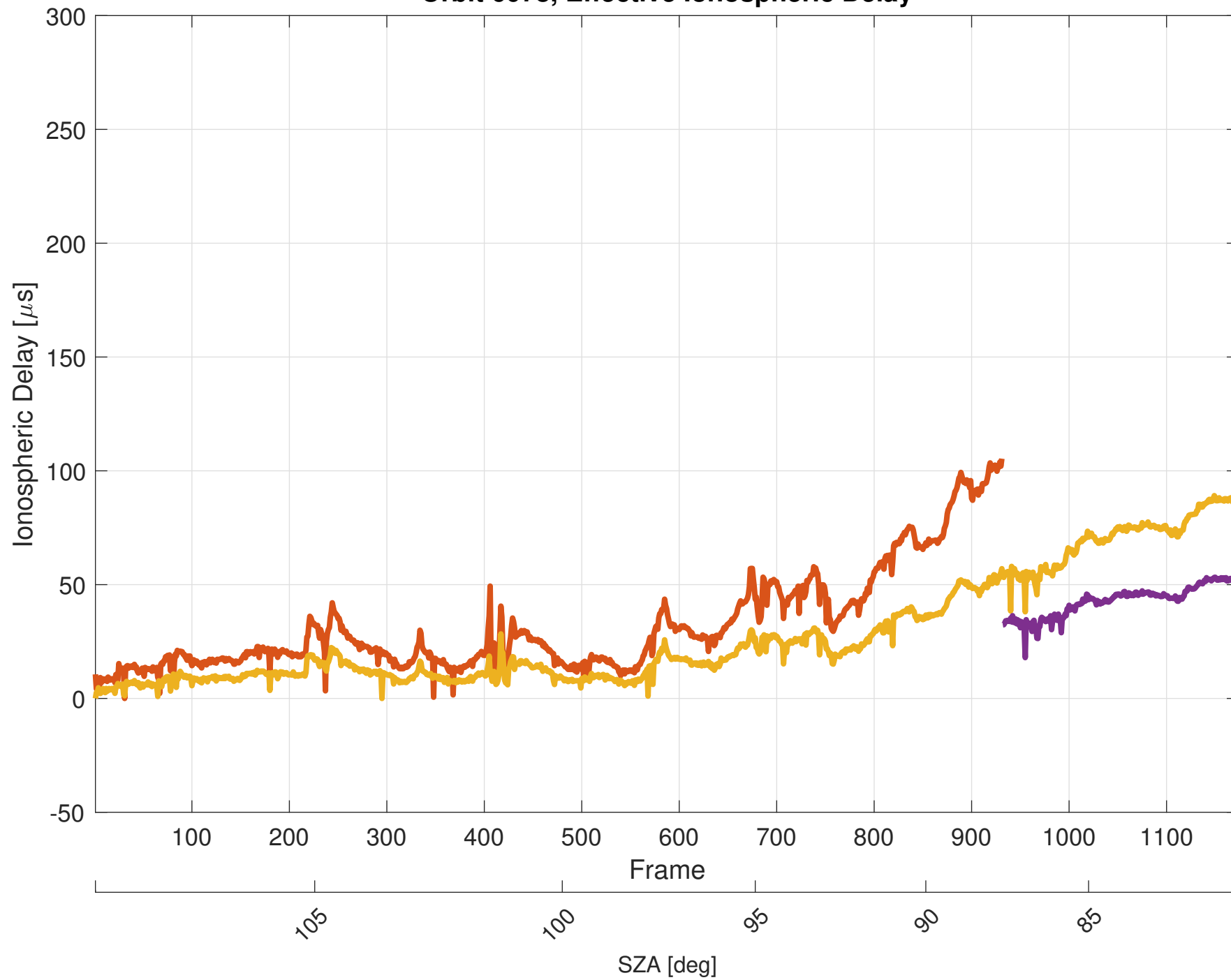
Orbit 6078, Effective Ionospheric Delay
