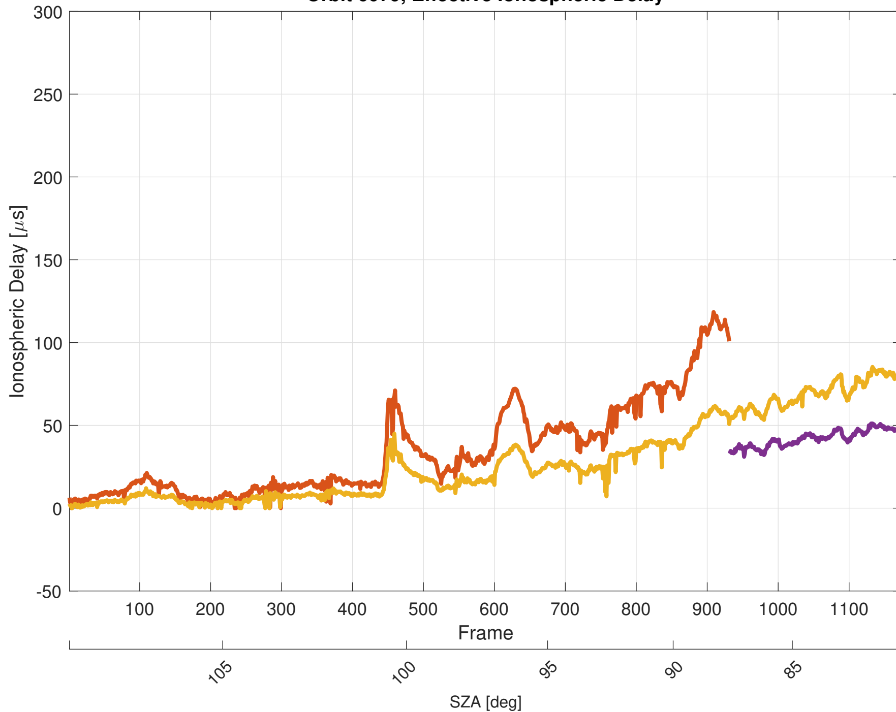
Orbit 6079, Effective Ionospheric Delay
