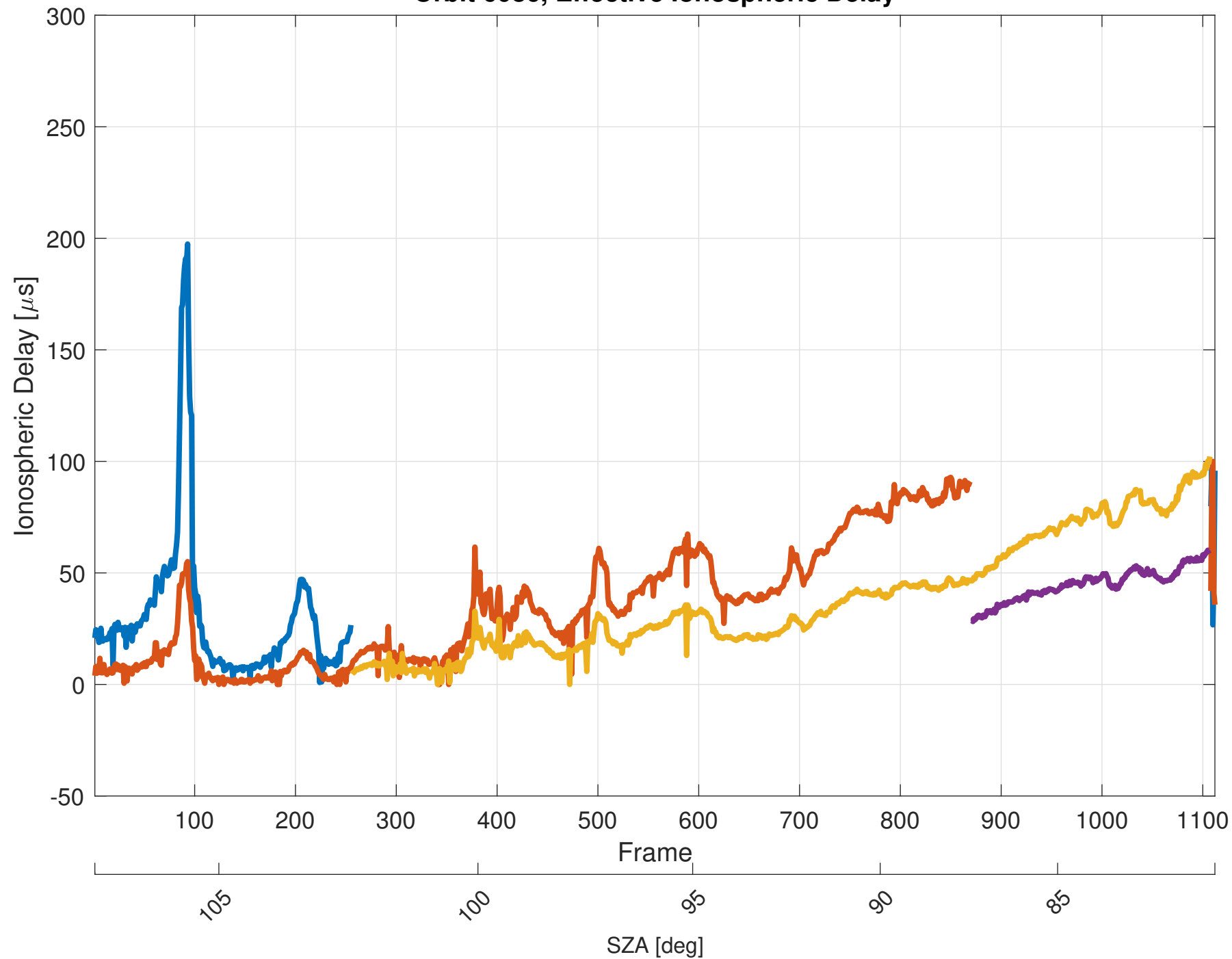
Orbit 6086, Effective Ionospheric Delay
