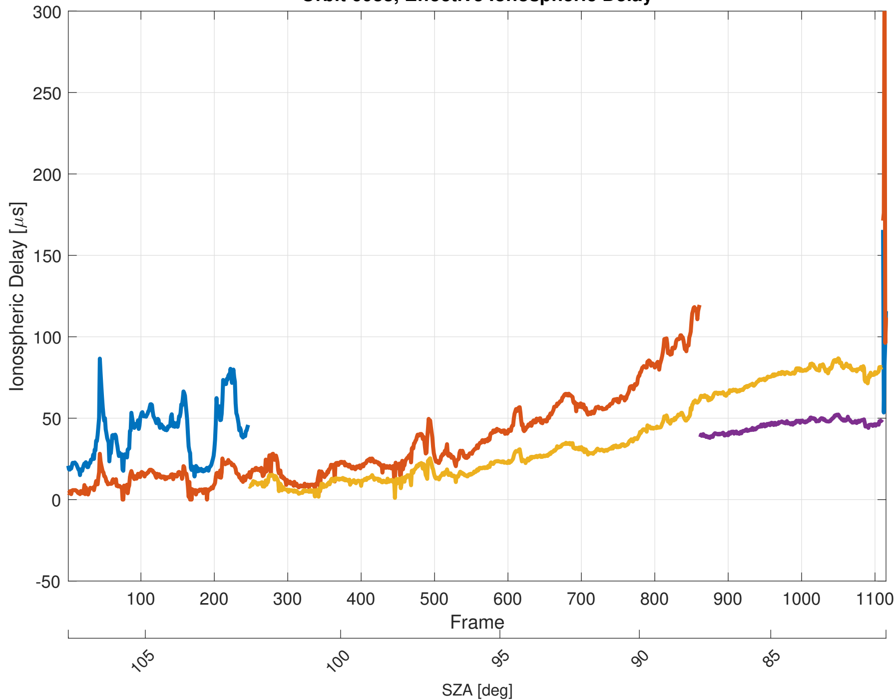
Orbit 6088, Effective Ionospheric Delay
