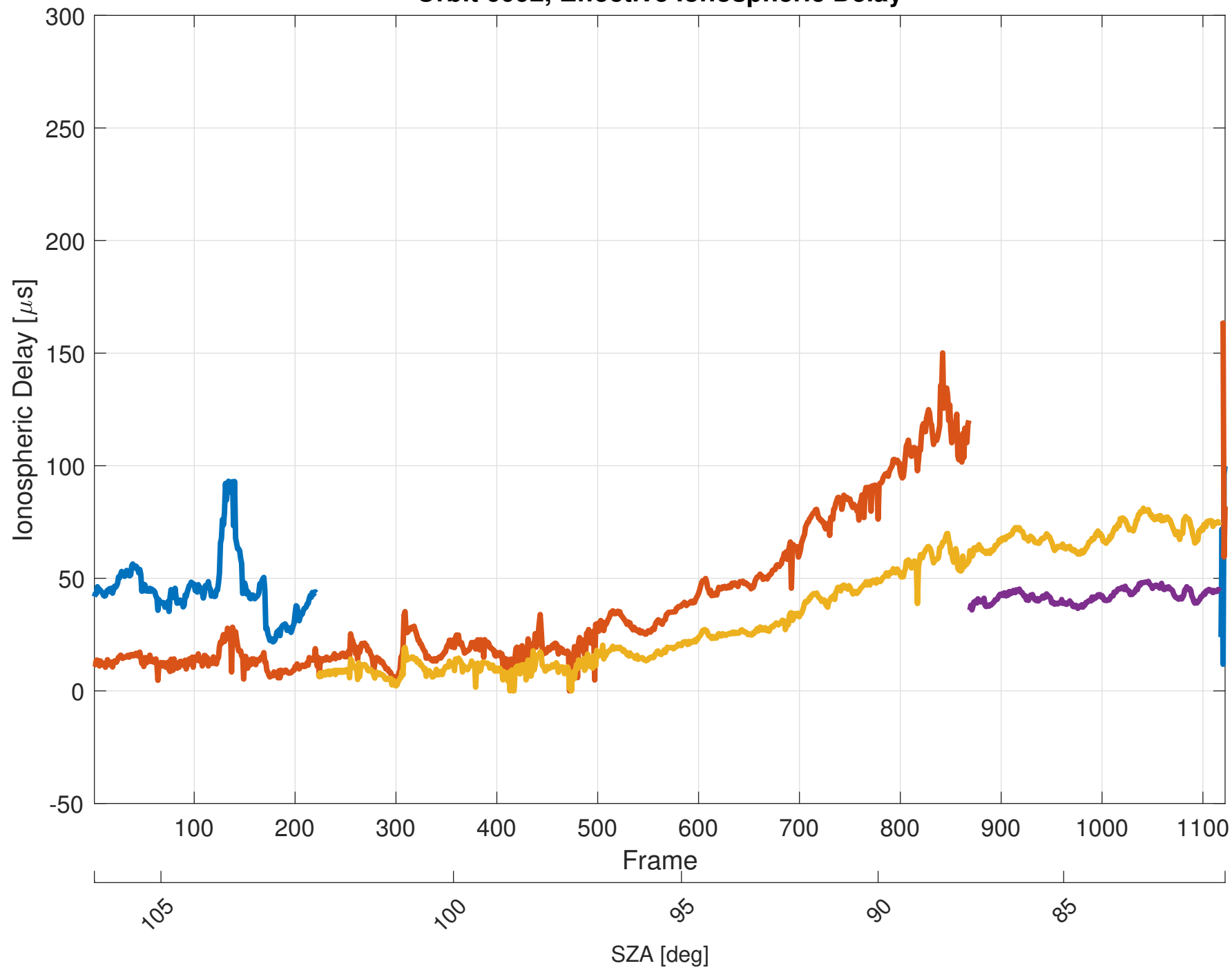
Orbit 6092, Effective Ionospheric Delay
