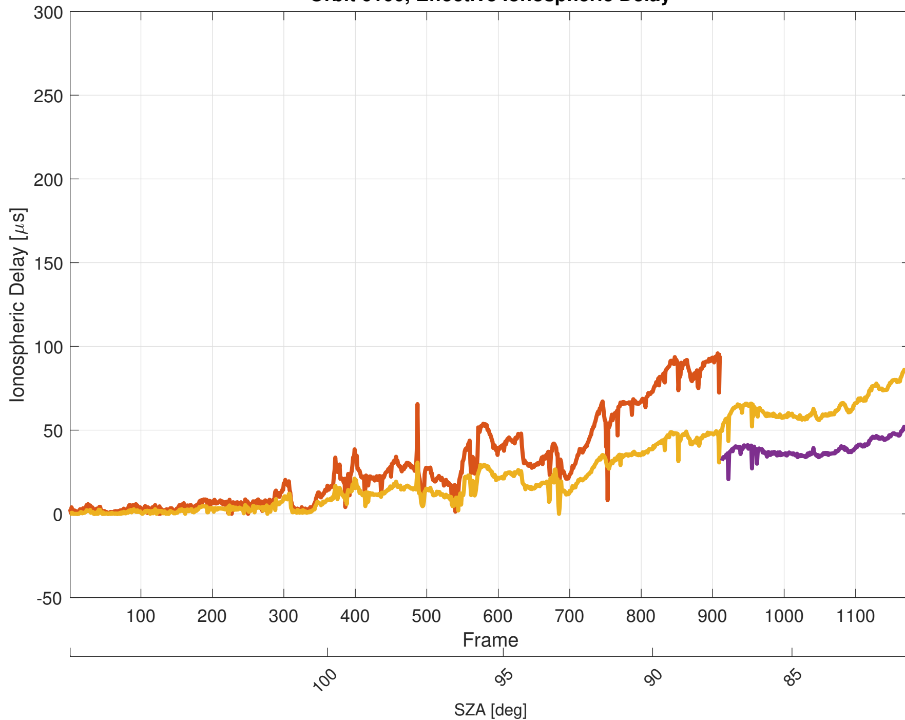
Orbit 6100, Effective Ionospheric Delay
