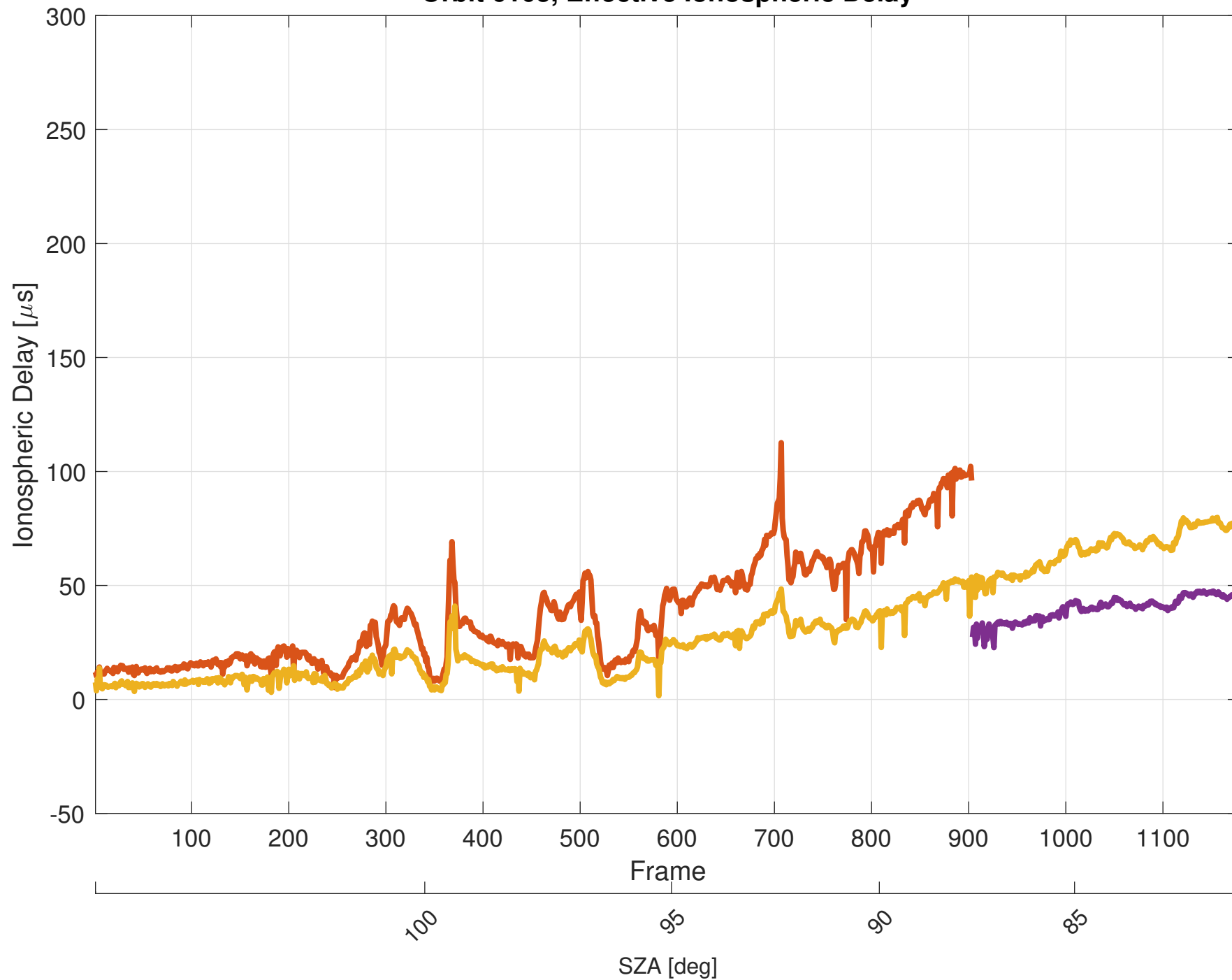
Orbit 6103, Effective Ionospheric Delay
