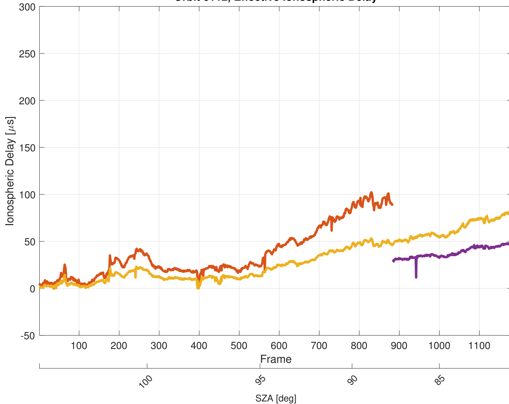
Orbit 6112, Effective Ionospheric Delay
