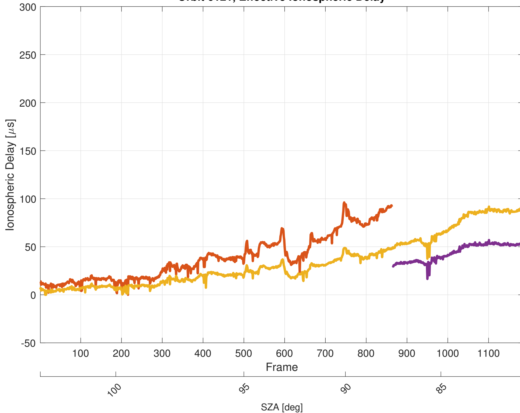
Orbit 6121, Effective Ionospheric Delay
