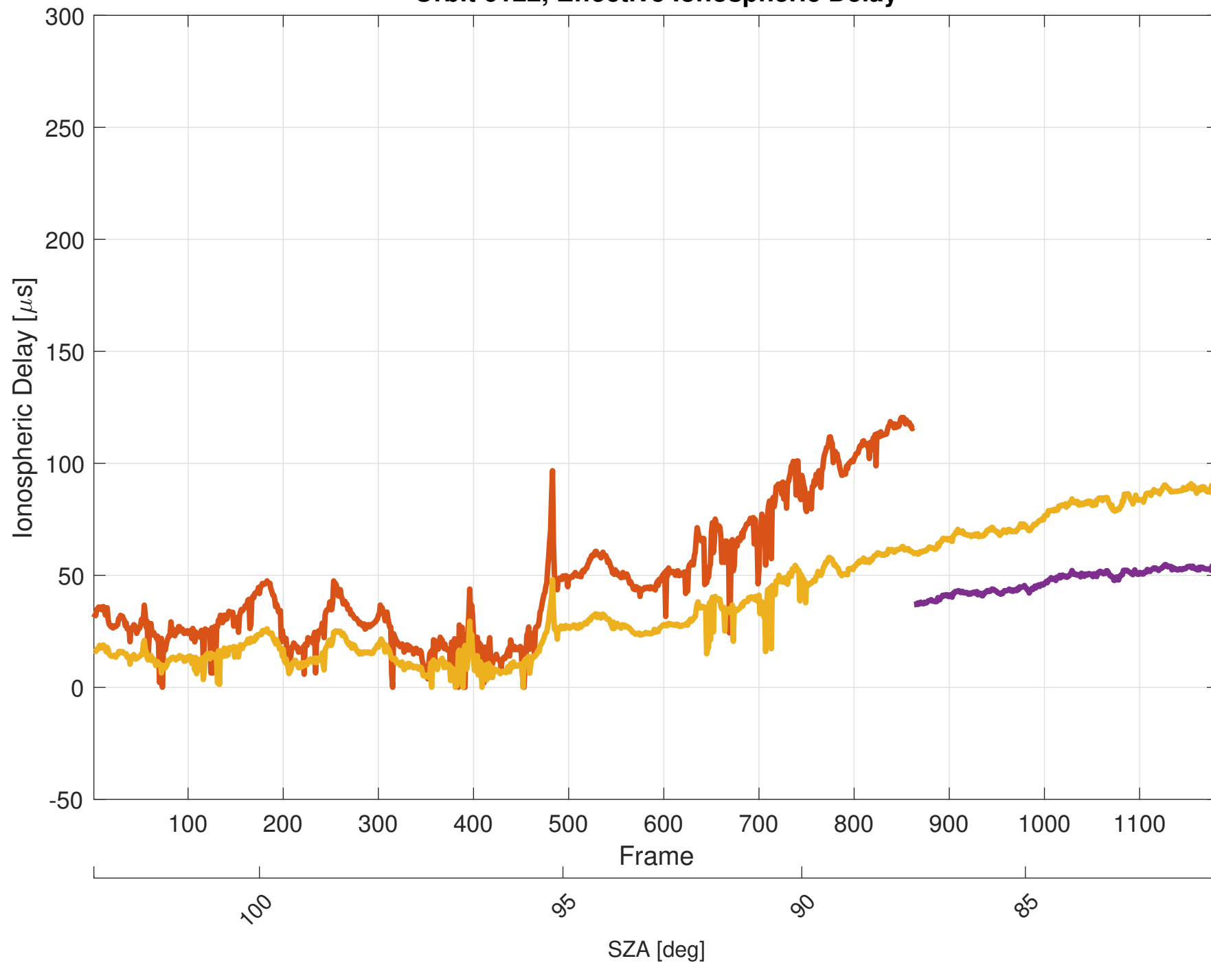
Orbit 6122, Effective Ionospheric Delay
