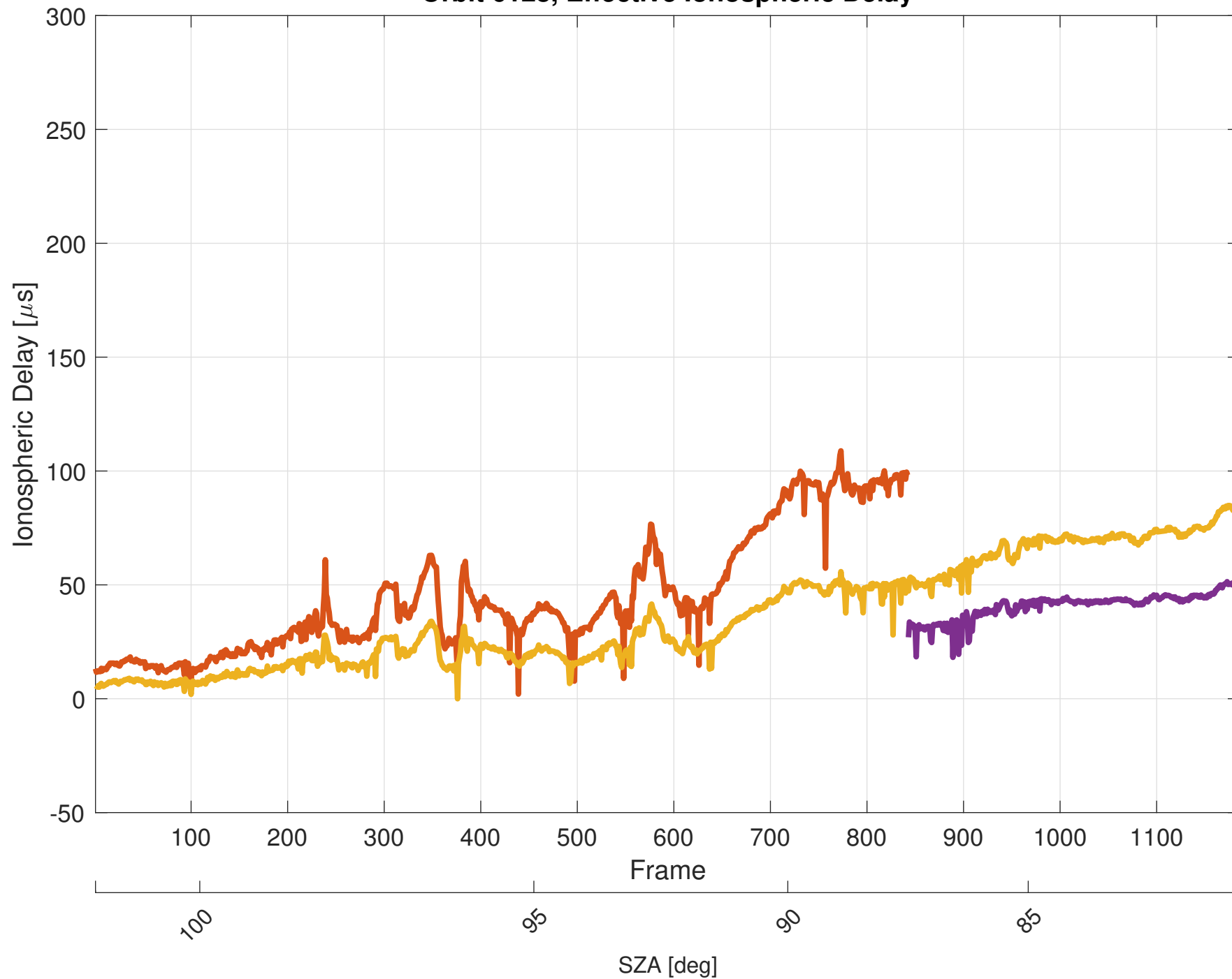
Orbit 6128, Effective Ionospheric Delay
