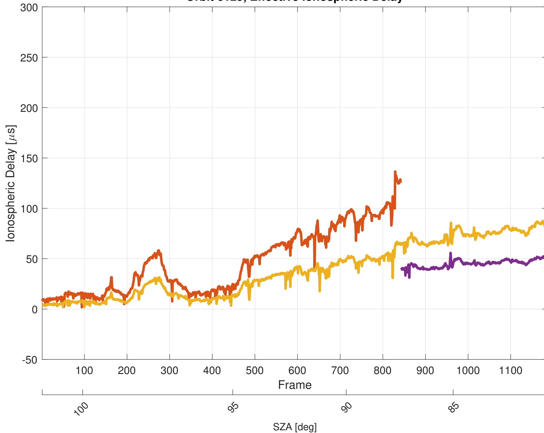
Orbit 6129, Effective Ionospheric Delay
