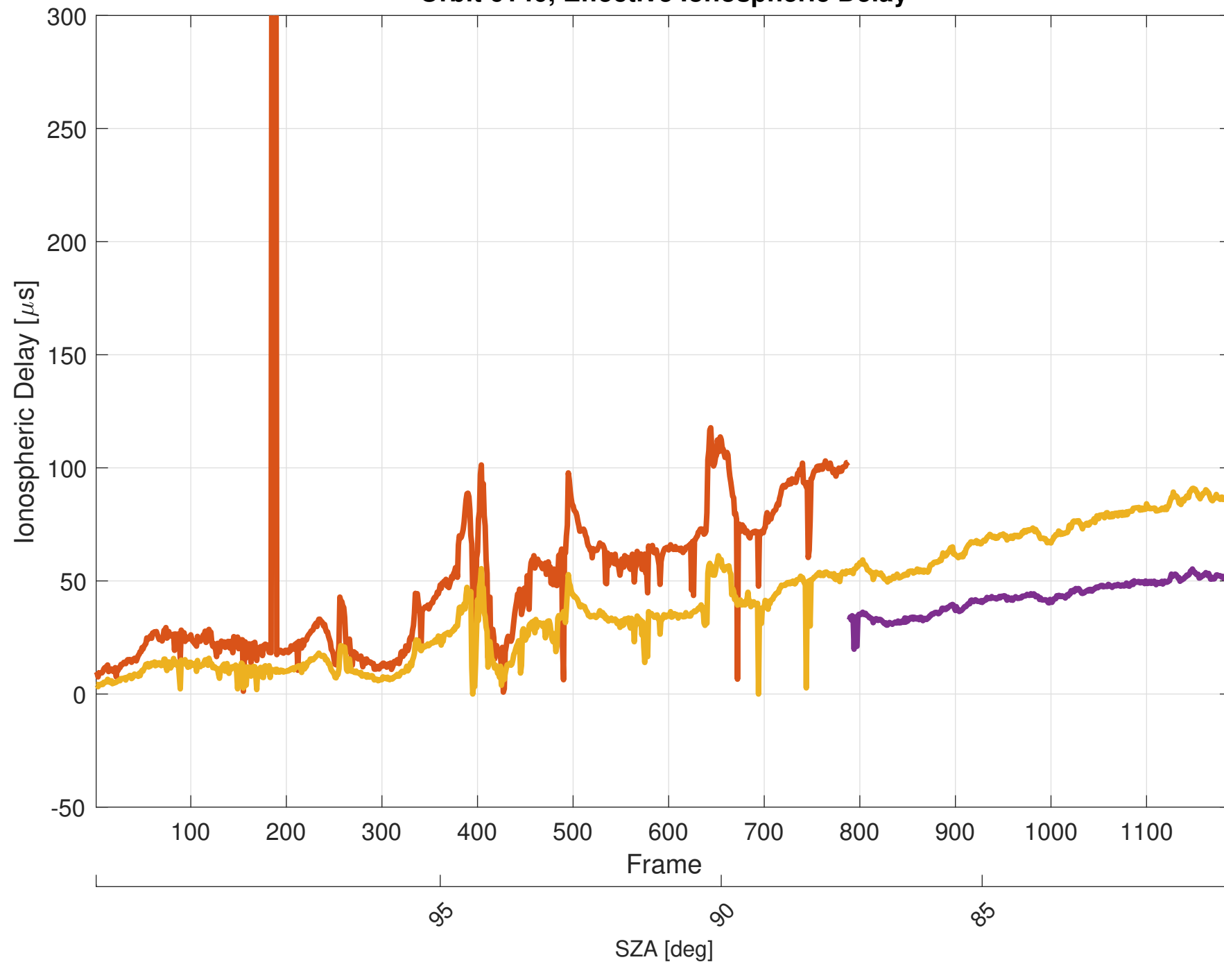
Orbit 6140, Effective Ionospheric Delay
