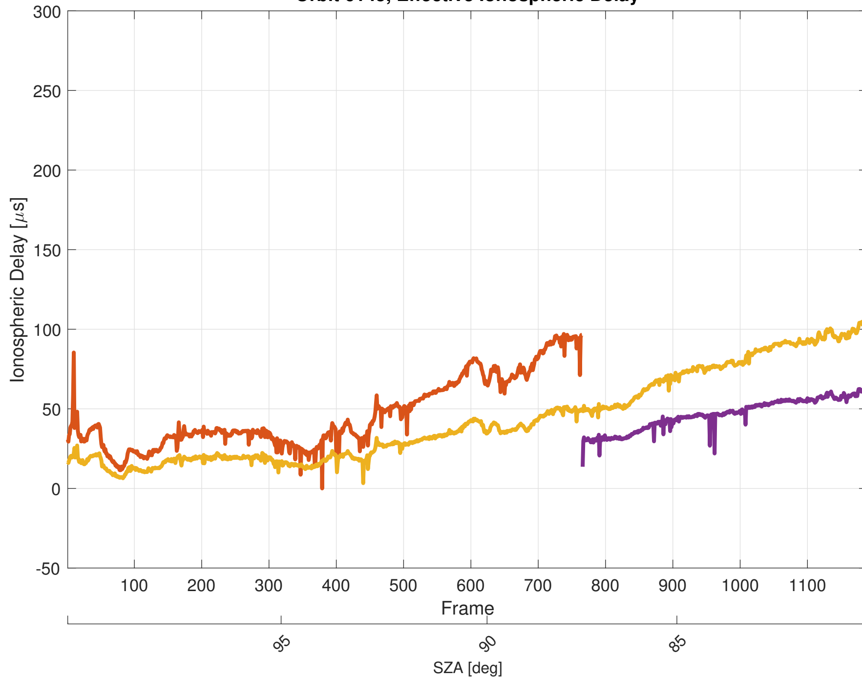
Orbit 6145, Effective Ionospheric Delay
