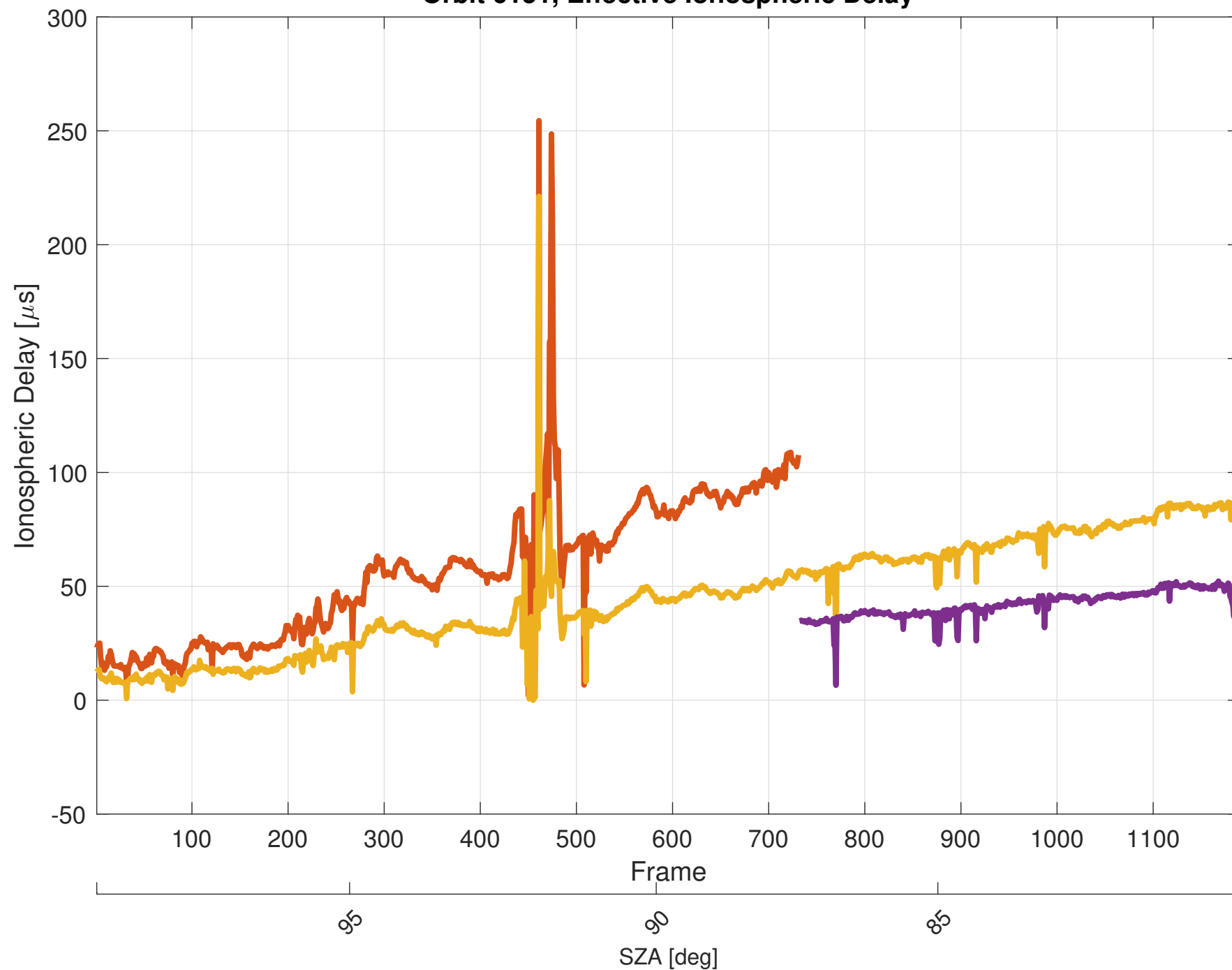
Orbit 6151, Effective Ionospheric Delay
