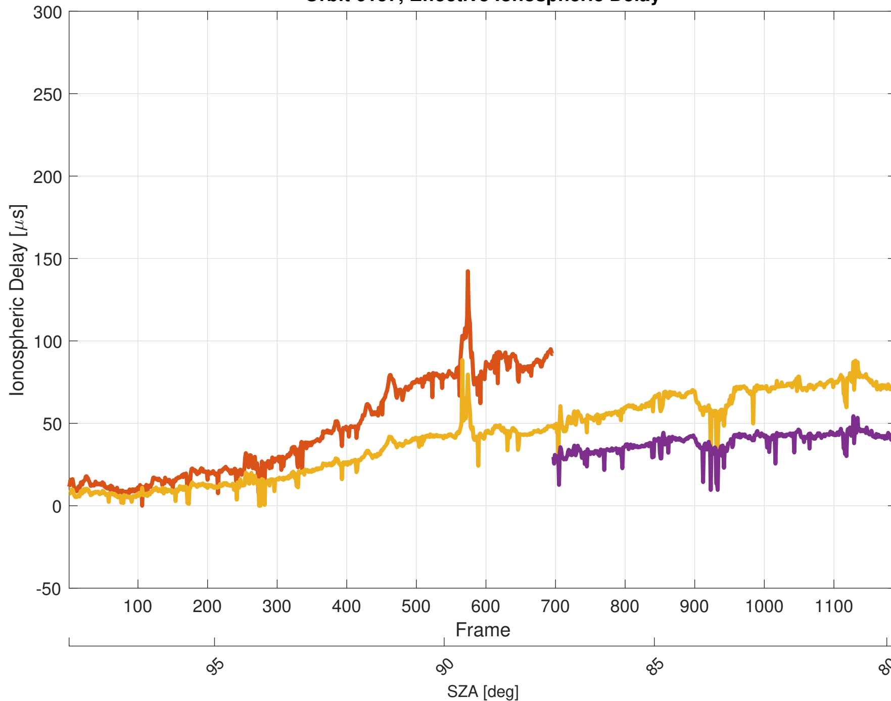
Orbit 6157, Effective Ionospheric Delay
