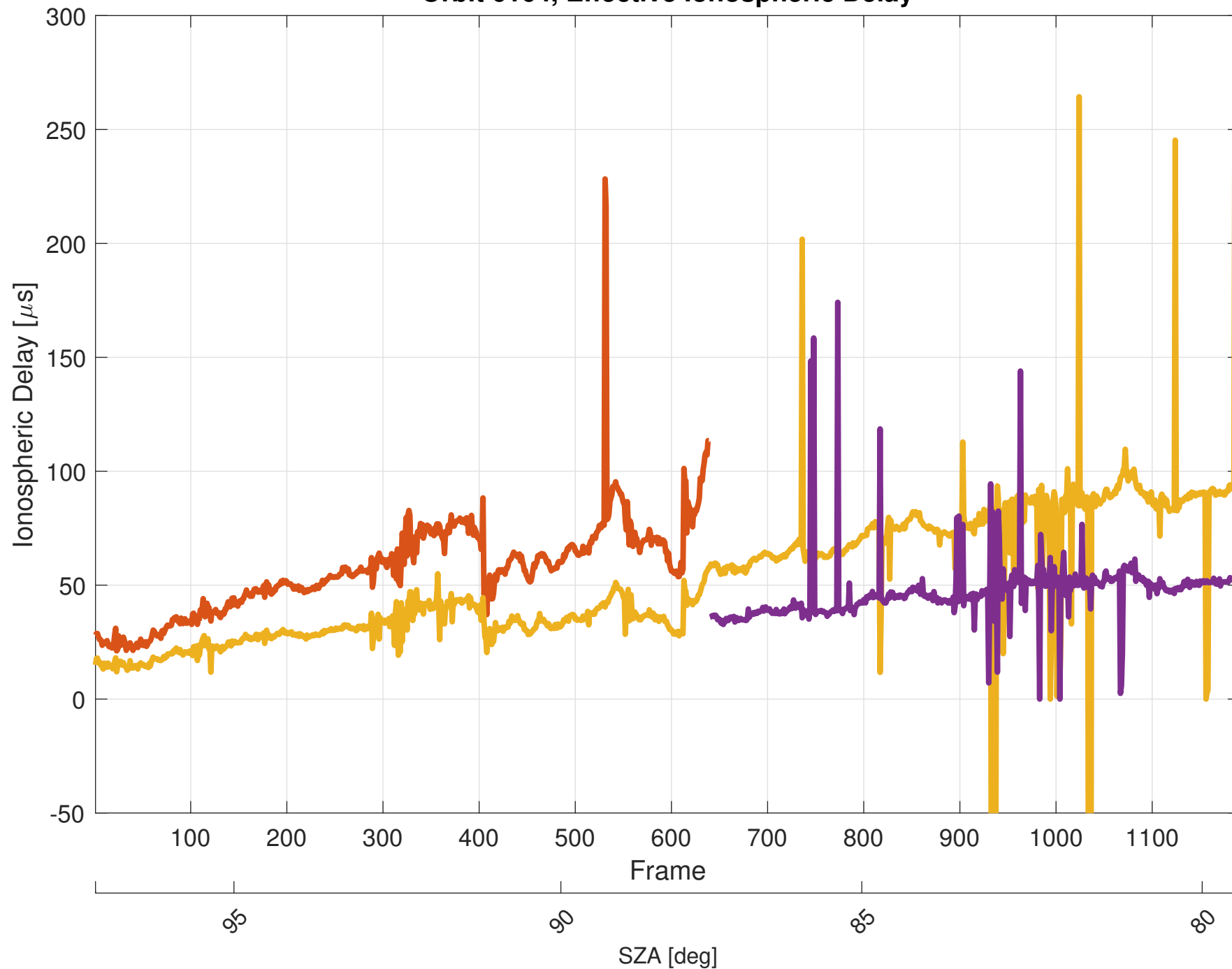
Orbit 6164, Effective Ionospheric Delay
