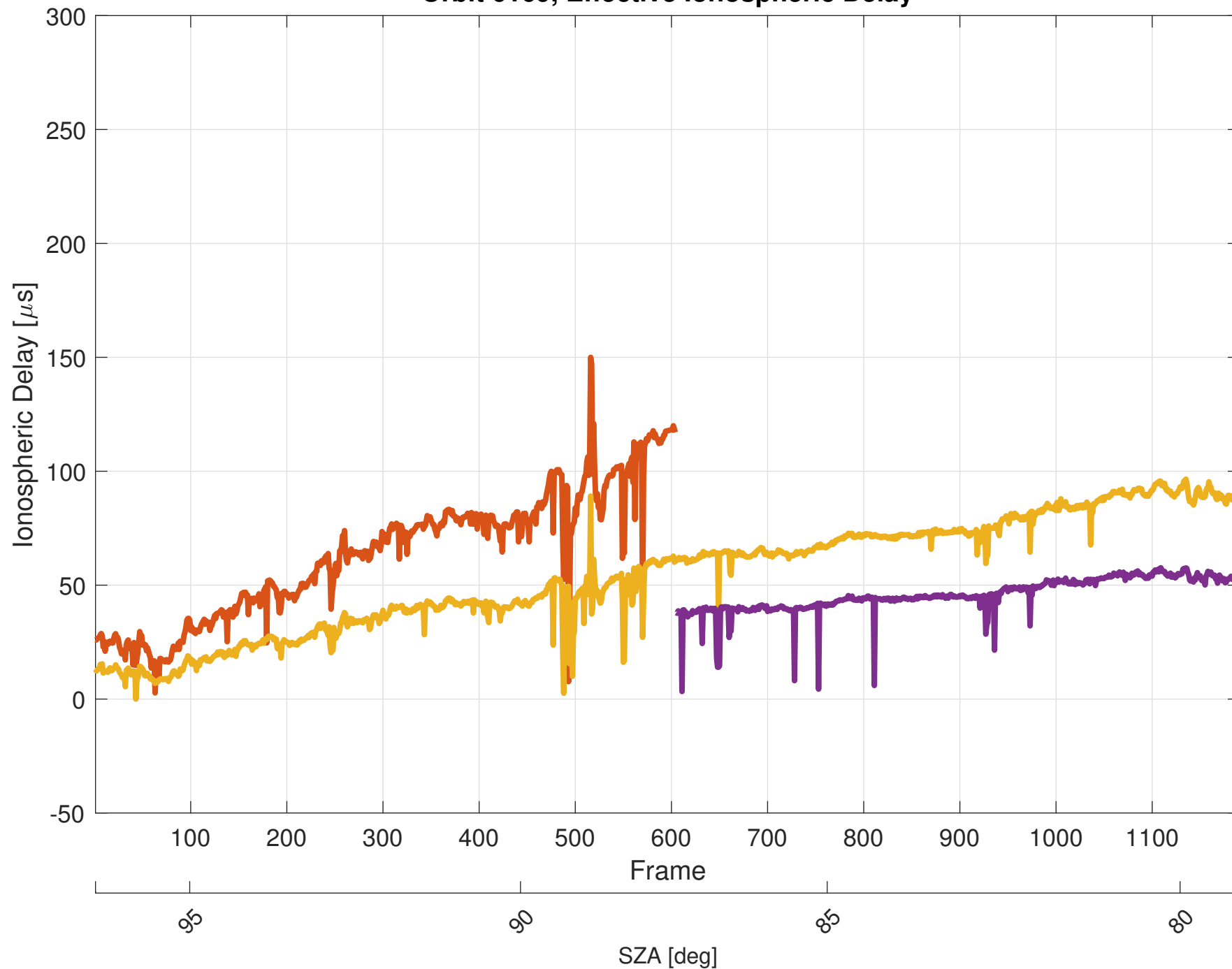
Orbit 6169, Effective Ionospheric Delay
