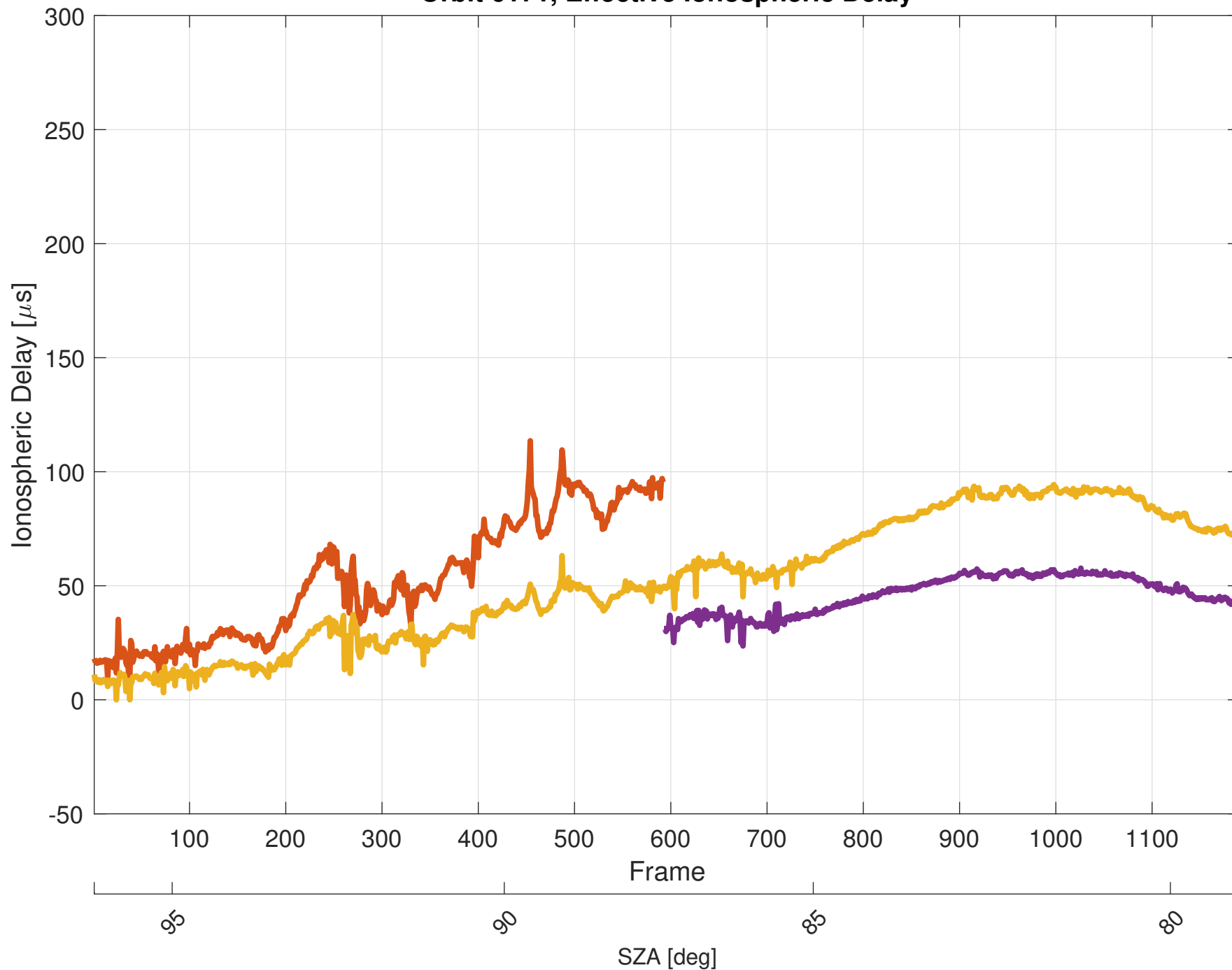
Orbit 6171, Effective Ionospheric Delay
