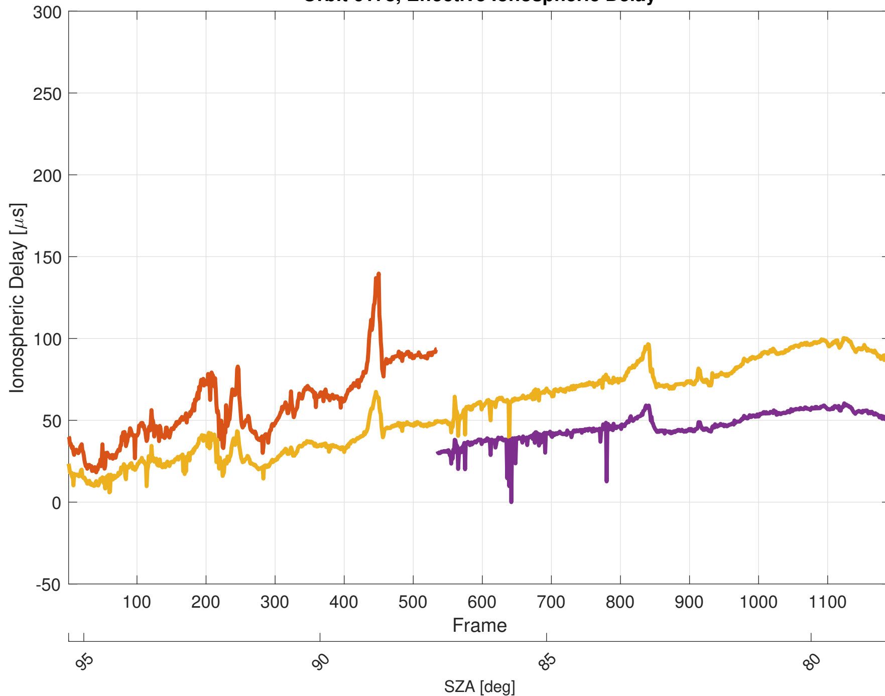
Orbit 6178, Effective Ionospheric Delay
