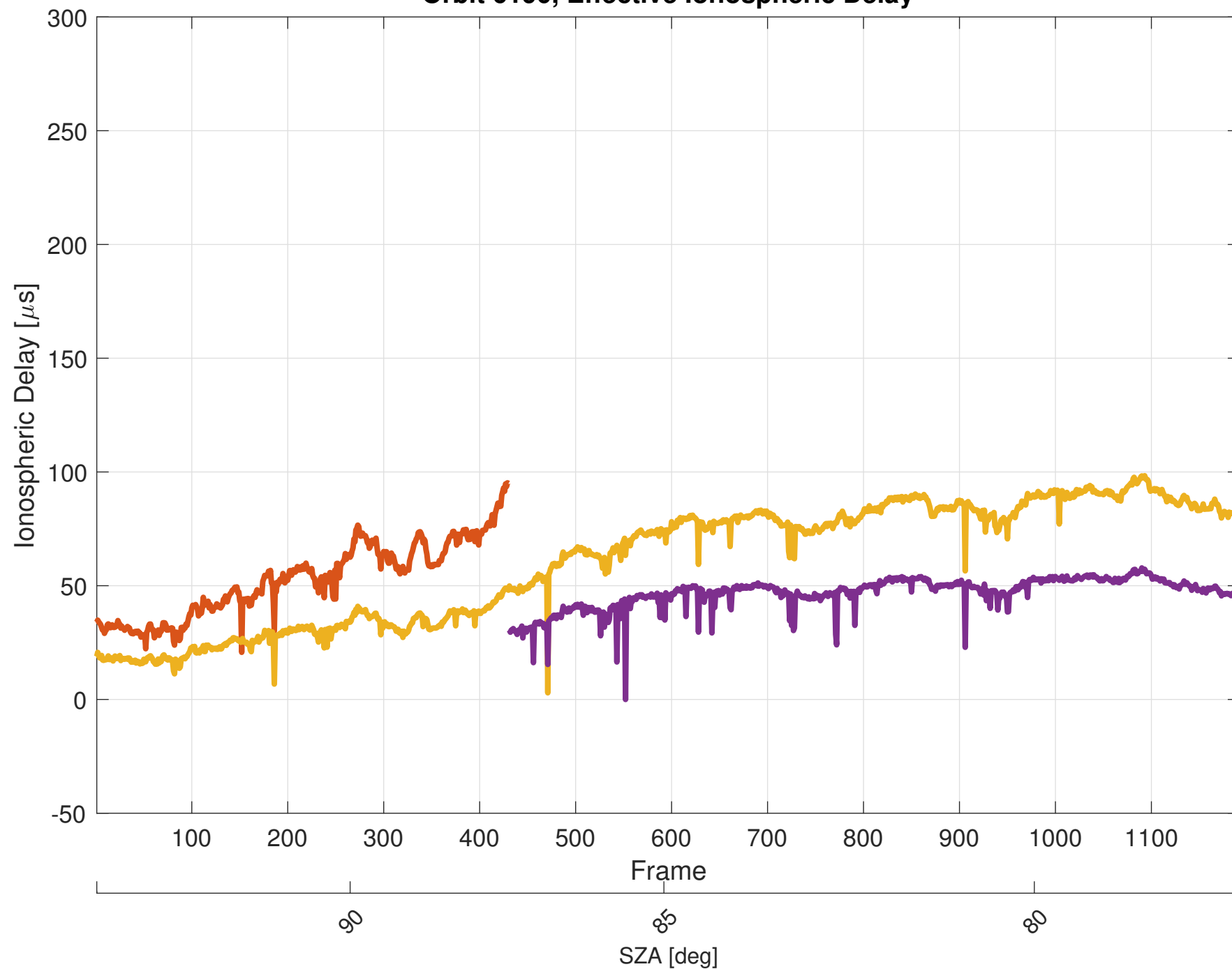
Orbit 6190, Effective Ionospheric Delay
