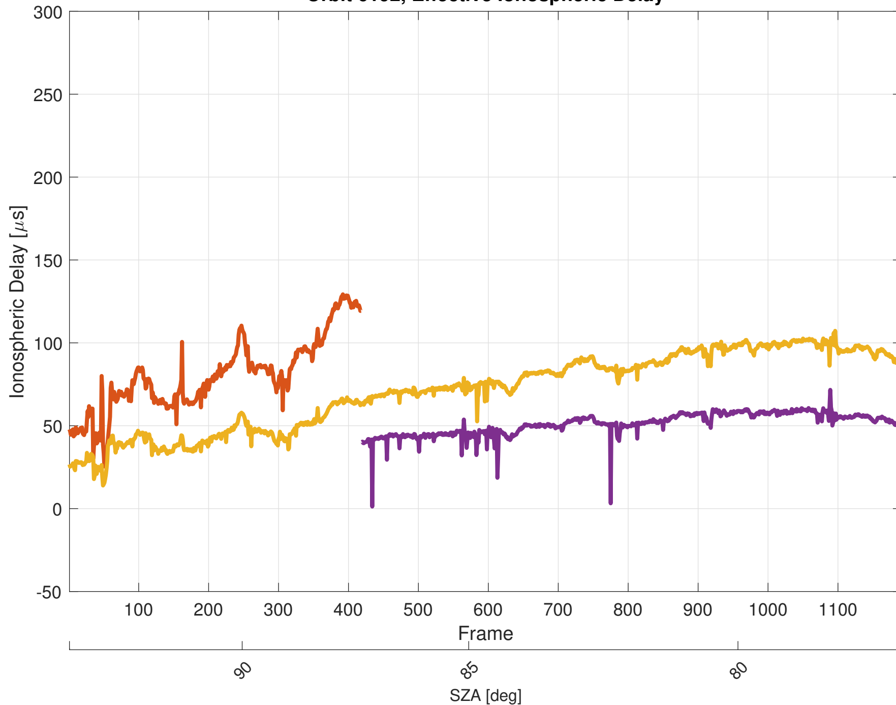
Orbit 6192, Effective Ionospheric Delay
