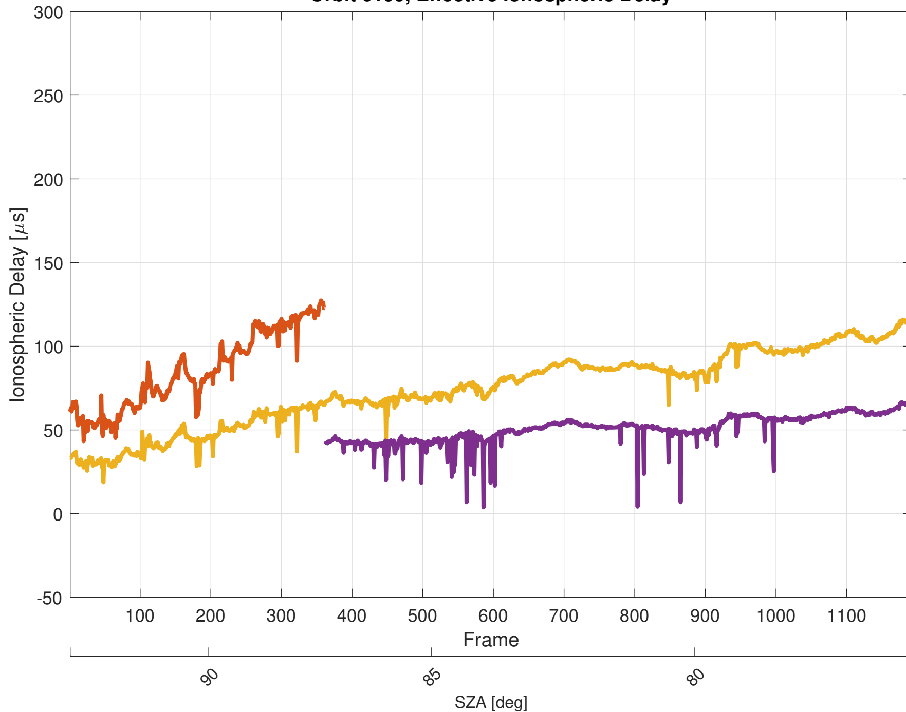
Orbit 6199, Effective Ionospheric Delay
