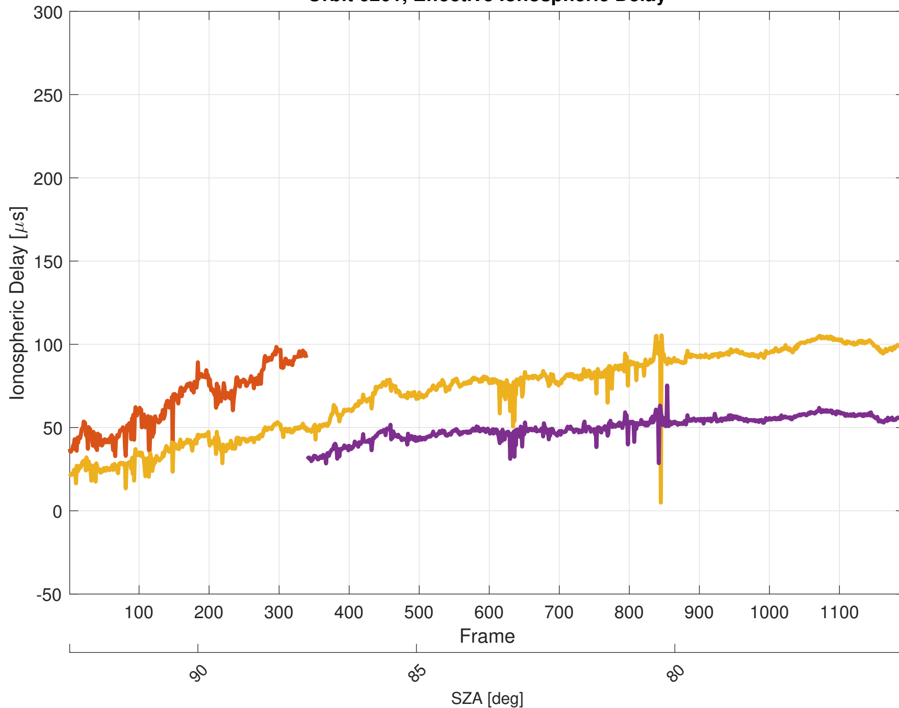
Orbit 6201, Effective Ionospheric Delay
