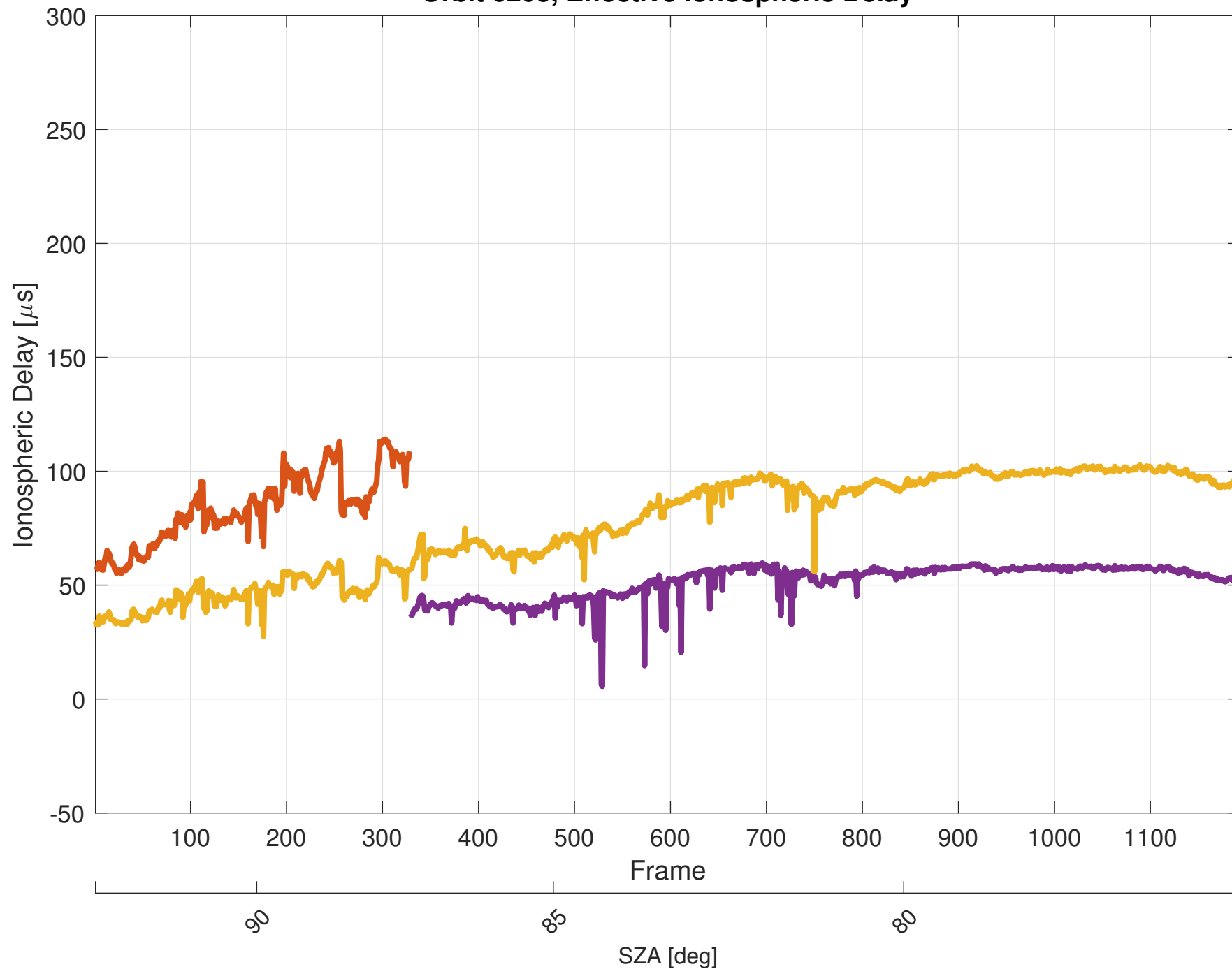
Orbit 6203, Effective Ionospheric Delay
