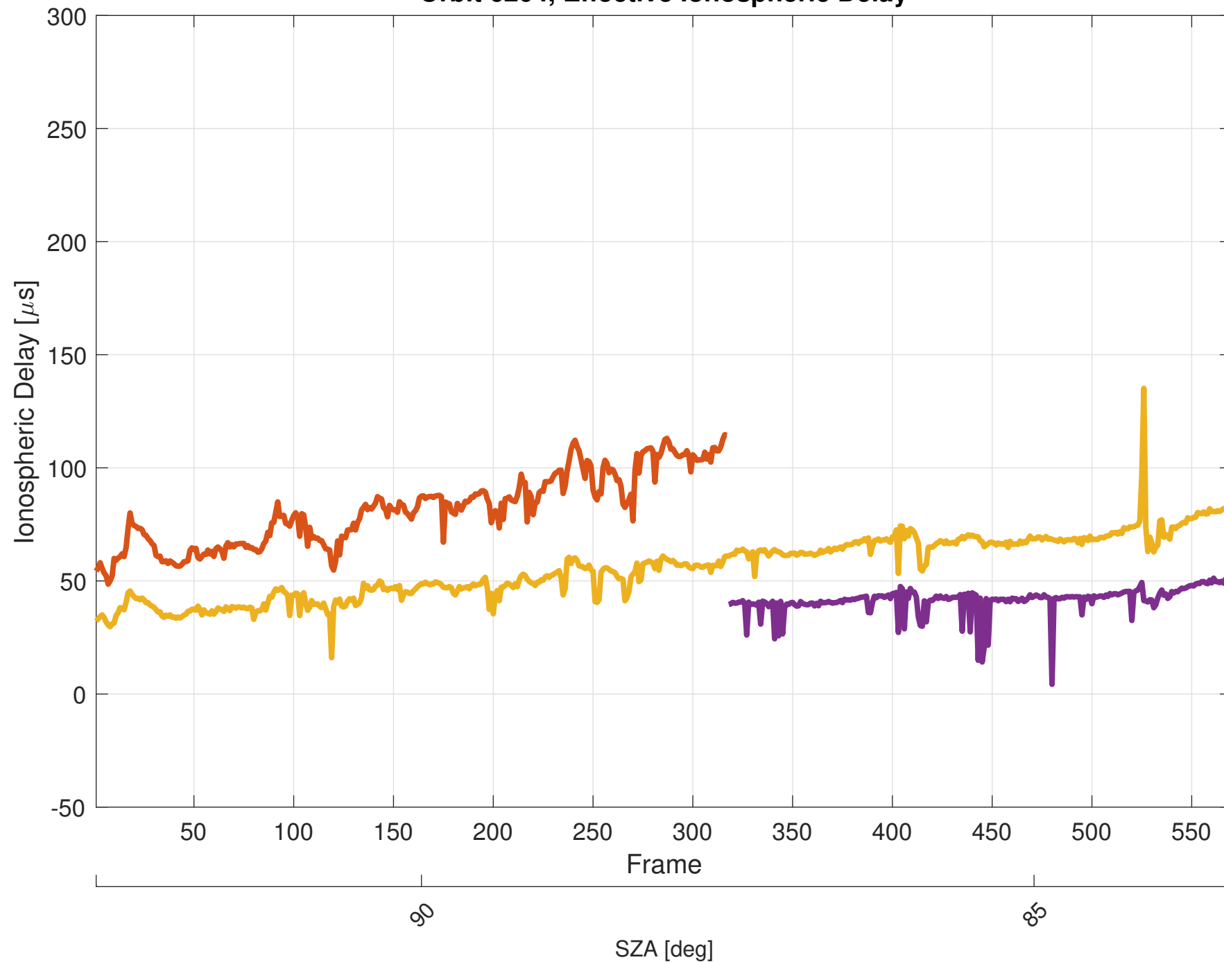
Orbit 6204, Effective Ionospheric Delay
