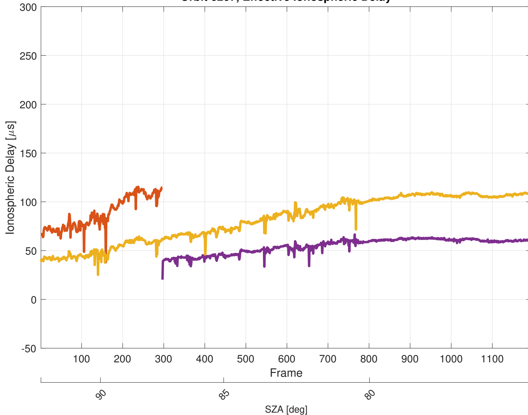
Orbit 6207, Effective Ionospheric Delay
